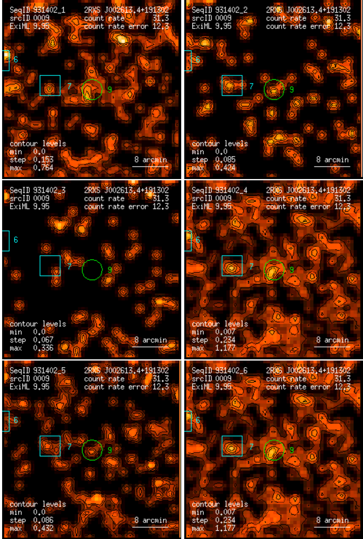
Figure 9: RASS 931402: detection 0009: band rate images, Gaussian filter: (1) PSPC channels 11 – 41, (2) 52 – 90, (3) 91 – 201, (4) 11 – 235, (5) 52 – 201, (6) 11 – 201. Broad band rates in counts/ks. Band rate contour levels in counts/ks/arcmin 2 .
