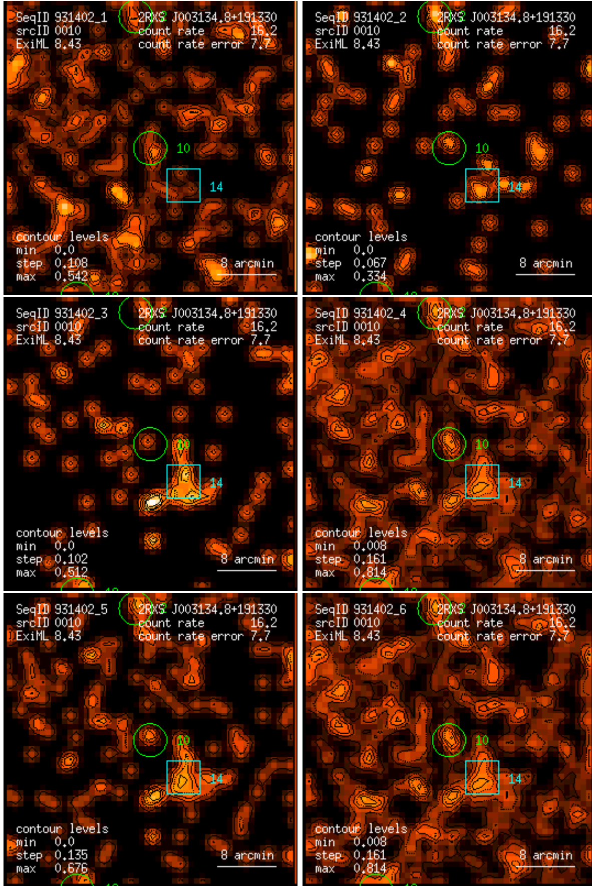
Figure 10: RASS 931402: detection 0010: band rate images, Gaussian filter: (1) PSPC channels 11 – 41, (2) 52 – 90, (3) 91 – 201, (4) 11 – 235, (5) 52 – 201, (6) 11 – 201. Broad band rates in counts/ks. Band rate contour levels in counts/ks/arcmin 2 .
