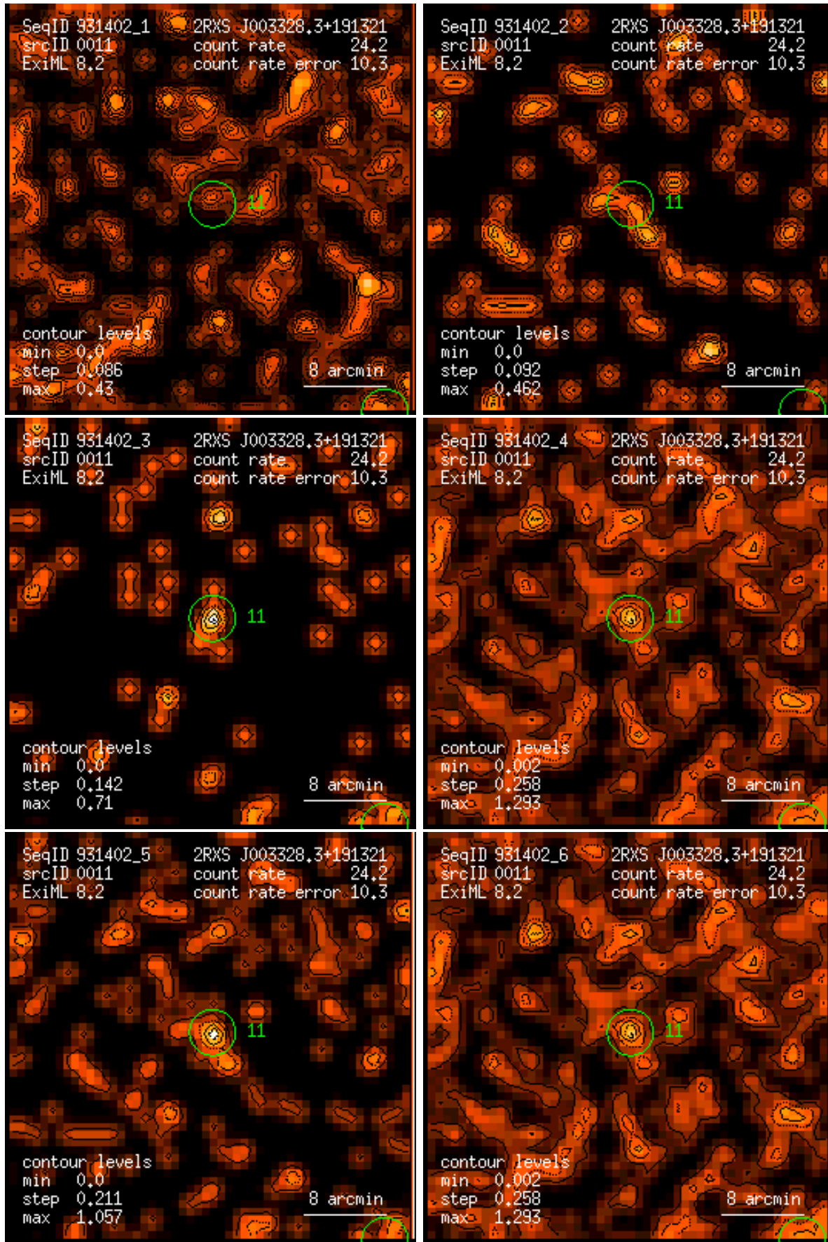
Figure 11: RASS 931402: detection 0011: band rate images, Gaussian filter: (1) PSPC channels 11 – 41, (2) 52 – 90, (3) 91 – 201, (4) 11 – 235, (5) 52 – 201, (6) 11 – 201. Broad band rates in counts/ks. Band rate contour levels in counts/ks/arcmin 2 .
