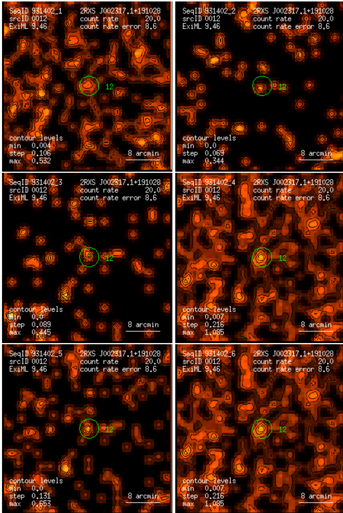
Figure 12: RASS 931402: detection 0012: band rate images, Gaussian filter: (1) PSPC channels 11 – 41, (2) 52 – 90, (3) 91 – 201, (4) 11 – 235, (5) 52 – 201, (6) 11 – 201. Broad band rates in counts/ks. Band rate contour levels in counts/ks/arcmin 2 .
