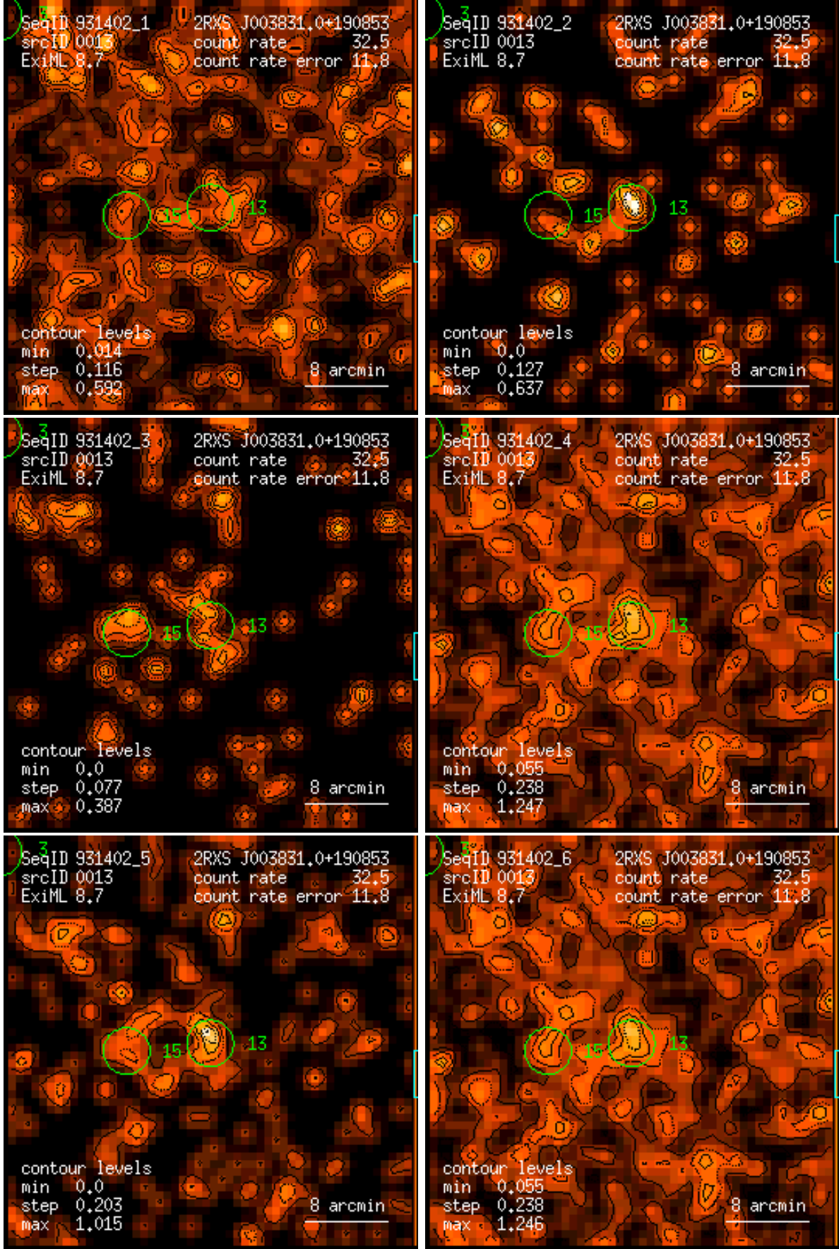
Figure 13: RASS 931402: detection 0013: band rate images, Gaussian filter: (1) PSPC channels 11 – 41, (2) 52 – 90, (3) 91 – 201, (4) 11 – 235, (5) 52 – 201, (6) 11 – 201. Broad band rates in counts/ks. Band rate contour levels in counts/ks/arcmin 2 .
