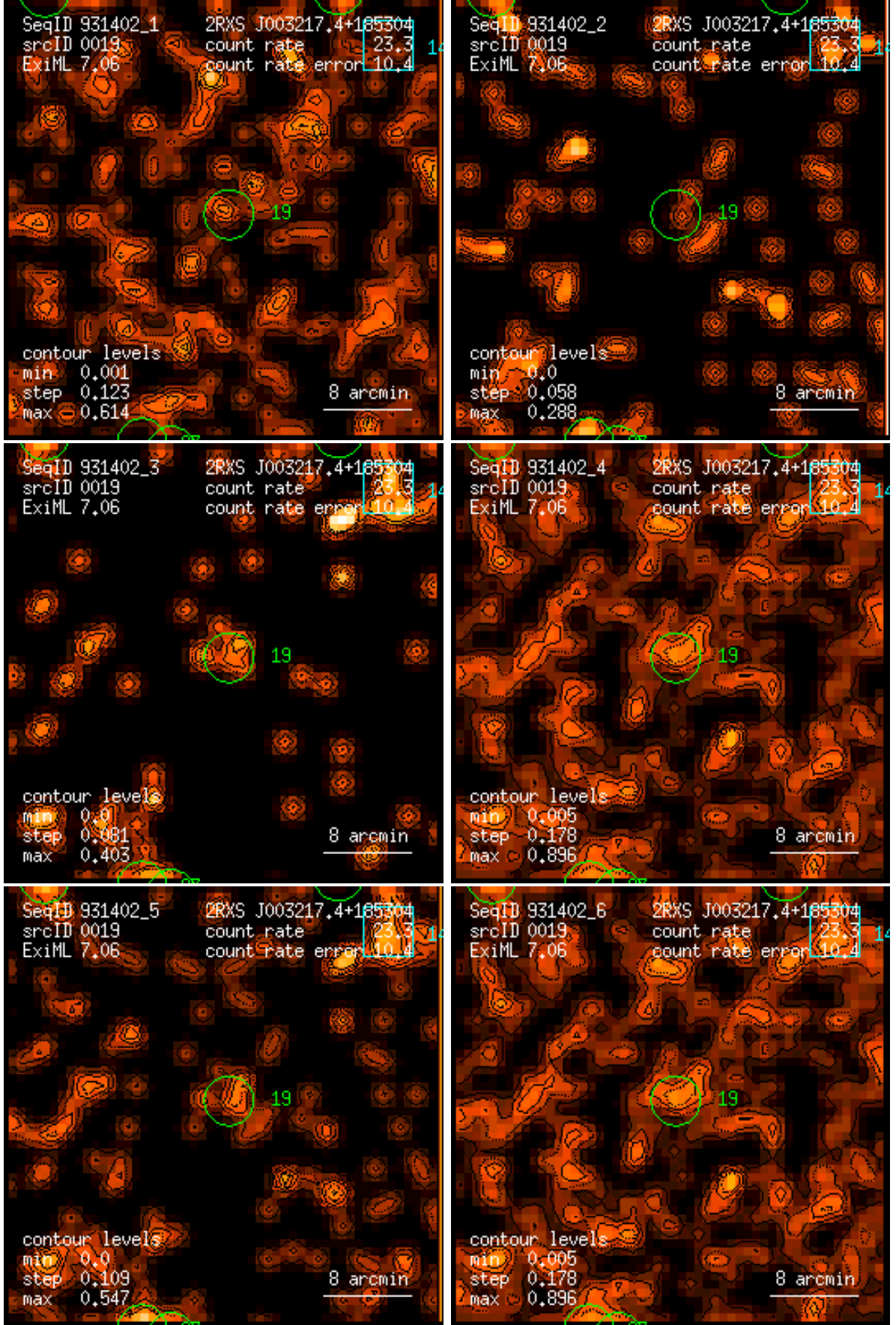
Figure 19: RASS 931402: detection 0019: band rate images, Gaussian filter: (1) PSPC channels 11 – 41, (2) 52 – 90, (3) 91 – 201, (4) 11 – 235, (5) 52 – 201, (6) 11 – 201. Broad band rates in counts/ks. Band rate contour levels in counts/ks/arcmin 2 .
