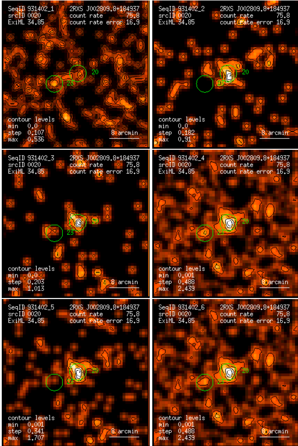
Figure 20: RASS 931402: detection 0020: band rate images, Gaussian filter: (1) PSPC channels 11 – 41, (2) 52 – 90, (3) 91 – 201, (4) 11 – 235, (5) 52 – 201, (6) 11 – 201. Broad band rates in counts/ks. Band rate contour levels in counts/ks/arcmin 2 .
