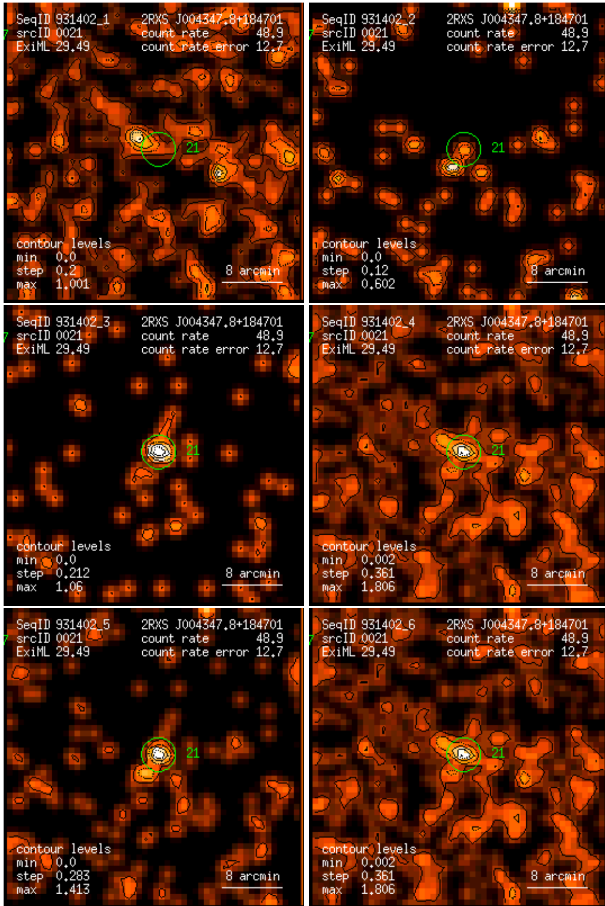
Figure 21: RASS 931402: detection 0021: band rate images, Gaussian filter: (1) PSPC channels 11 – 41, (2) 52 – 90, (3) 91 – 201, (4) 11 – 235, (5) 52 – 201, (6) 11 – 201. Broad band rates in counts/ks. Band rate contour levels in counts/ks/arcmin 2 .
