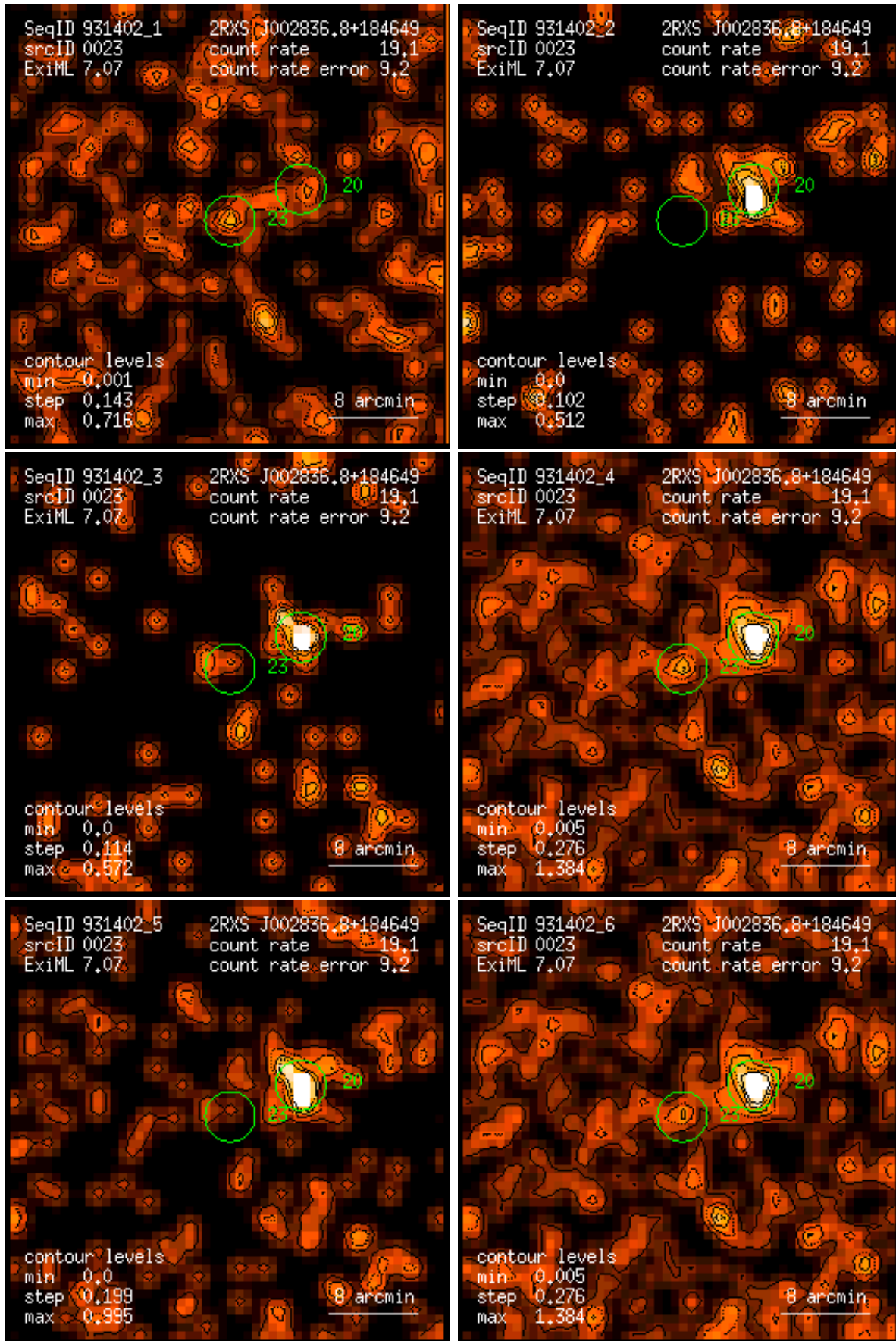
Figure 23: RASS 931402: detection 0023: band rate images, Gaussian filter: (1) PSPC channels 11 – 41, (2) 52 – 90, (3) 91 – 201, (4) 11 – 235, (5) 52 – 201, (6) 11 – 201. Broad band rates in counts/ks. Band rate contour levels in counts/ks/arcmin 2 .
