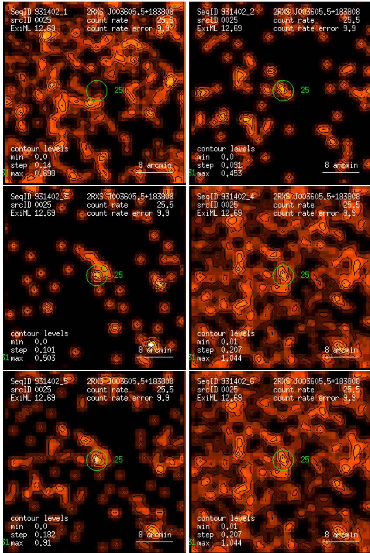
Figure 25: RASS 931402: detection 0025: band rate images, Gaussian filter: (1) PSPC channels 11 – 41, (2) 52 – 90, (3) 91 – 201, (4) 11 – 235, (5) 52 – 201, (6) 11 – 201. Broad band rates in counts/ks. Band rate contour levels in counts/ks/arcmin 2 .
