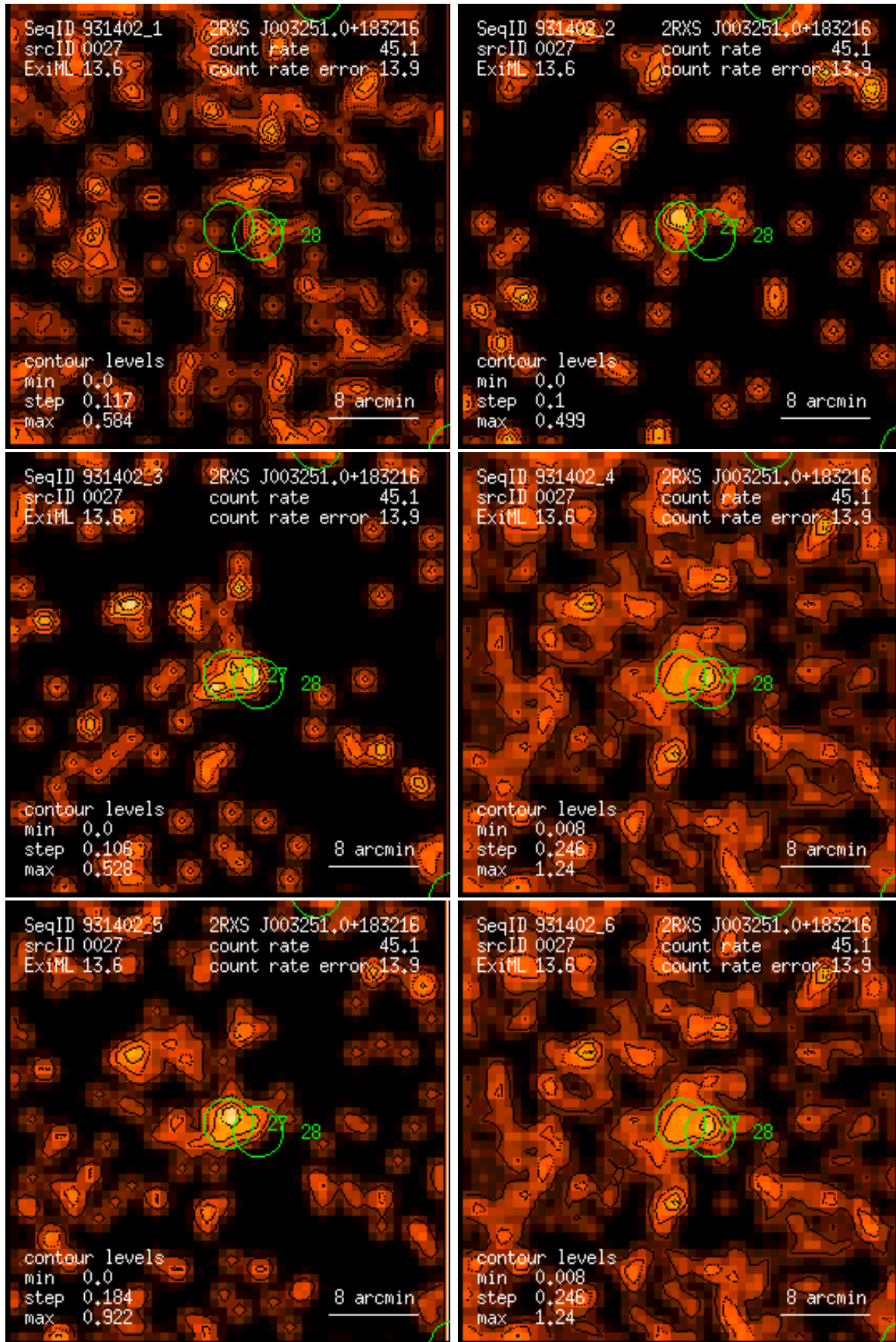
Figure 27: RASS 931402: detection 0027: band rate images, Gaussian filter: (1) PSPC channels 11 – 41, (2) 52 – 90, (3) 91 – 201, (4) 11 – 235, (5) 52 – 201, (6) 11 – 201. Broad band rates in counts/ks. Band rate contour levels in counts/ks/arcmin 2 .
