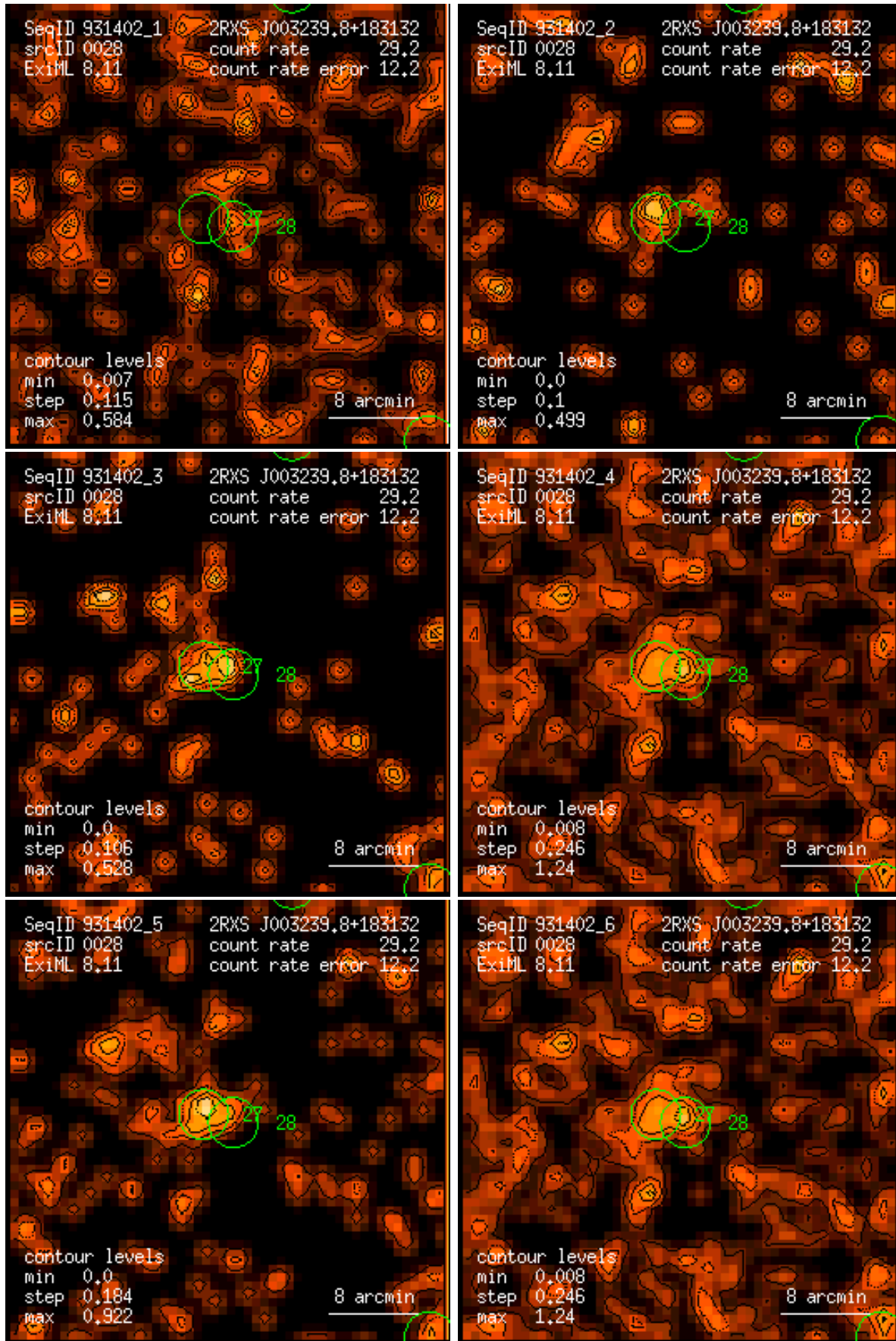
Figure 28: RASS 931402: detection 0028: band rate images, Gaussian filter: (1) PSPC channels 11 – 41, (2) 52 – 90, (3) 91 – 201, (4) 11 – 235, (5) 52 – 201, (6) 11 – 201. Broad band rates in counts/ks. Band rate contour levels in counts/ks/arcmin 2 .
