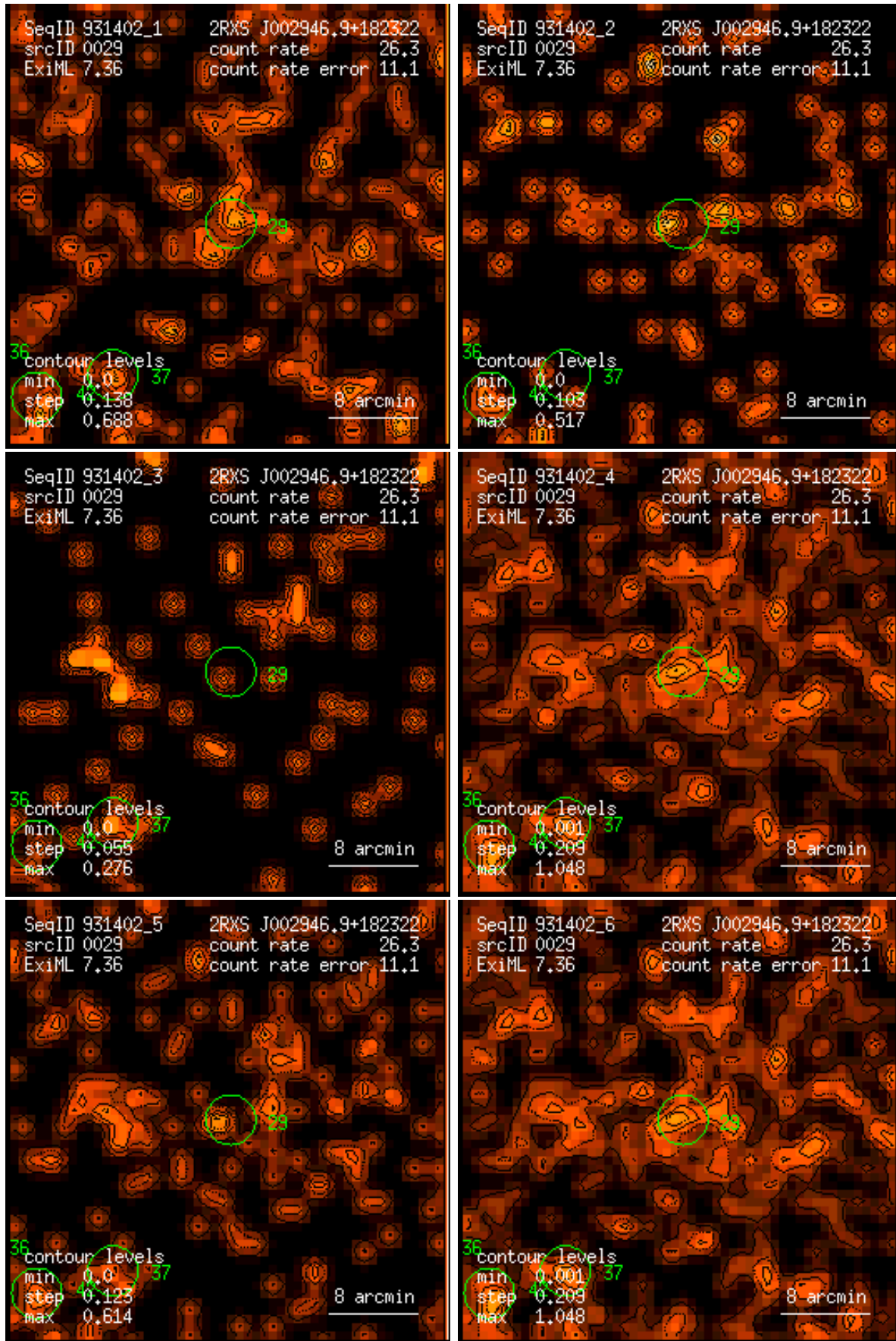
Figure 29: RASS 931402: detection 0029: band rate images, Gaussian filter: (1) PSPC channels 11 – 41, (2) 52 – 90, (3) 91 – 201, (4) 11 – 235, (5) 52 – 201, (6) 11 – 201. Broad band rates in counts/ks. Band rate contour levels in counts/ks/arcmin 2 .
