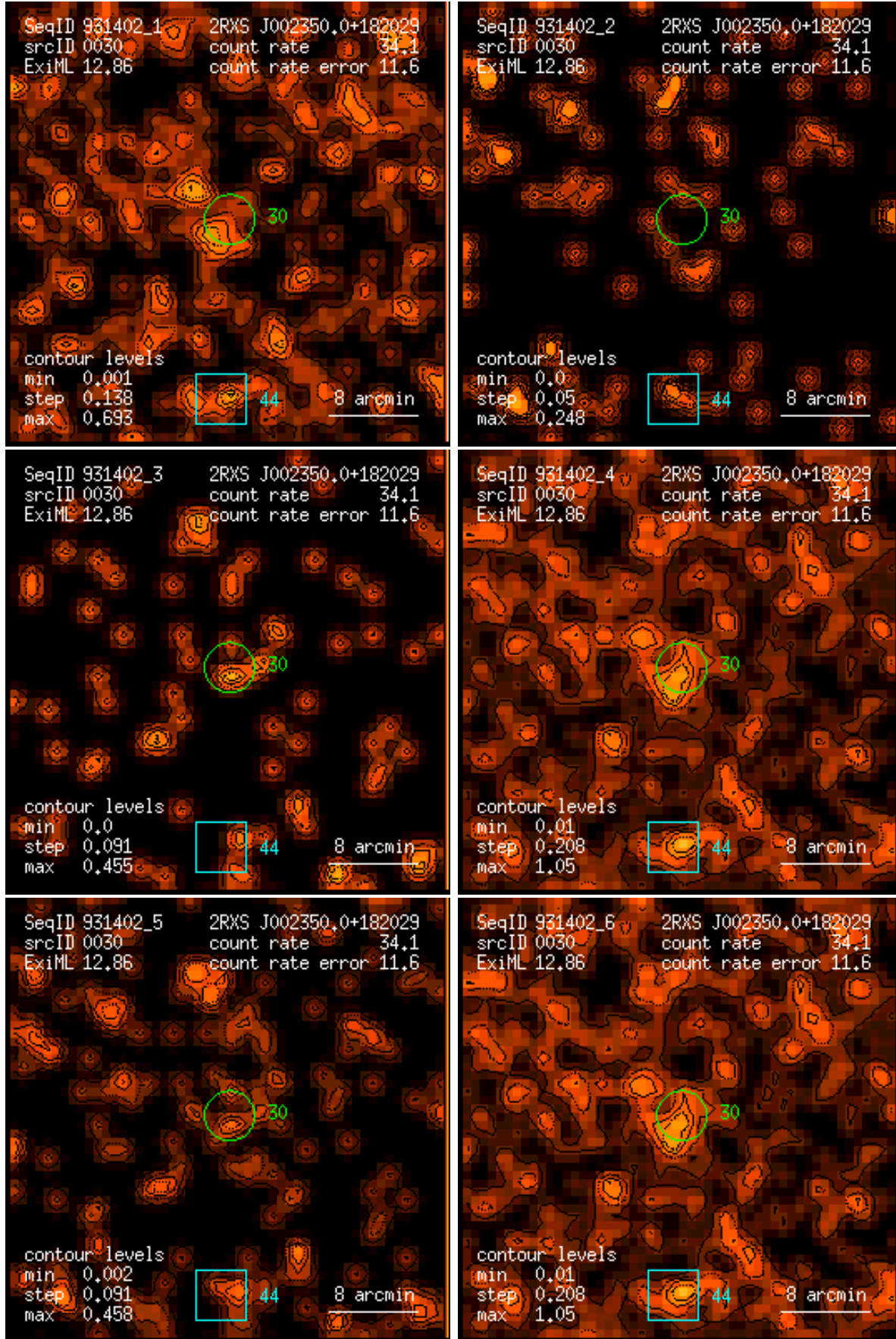
Figure 30: RASS 931402: detection 0030: band rate images, Gaussian filter: (1) PSPC channels 11 – 41, (2) 52 – 90, (3) 91 – 201, (4) 11 – 235, (5) 52 – 201, (6) 11 – 201. Broad band rates in counts/ks. Band rate contour levels in counts/ks/arcmin 2 .
