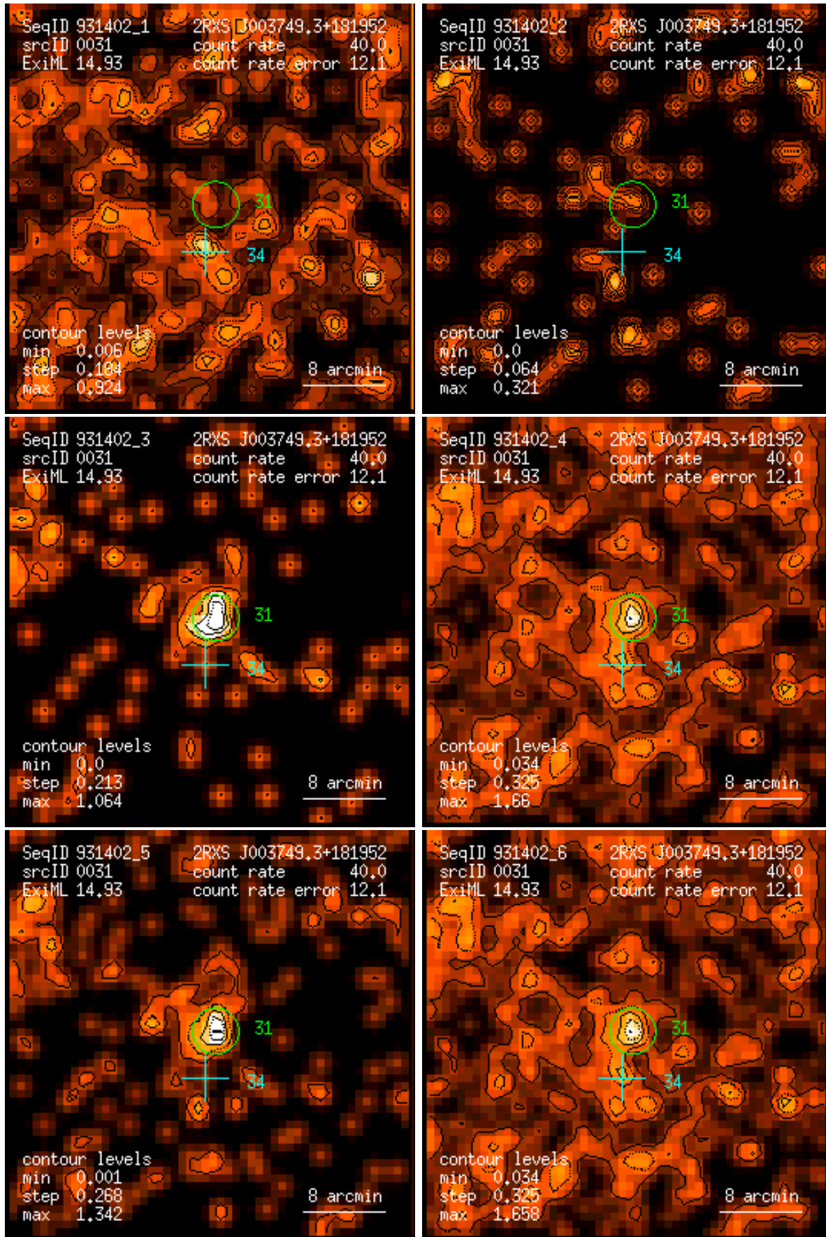
Figure 31: RASS 931402: detection 0031: band rate images, Gaussian filter: (1) PSPC channels 11 – 41, (2) 52 – 90, (3) 91 – 201, (4) 11 – 235, (5) 52 – 201, (6) 11 – 201. Broad band rates in counts/ks. Band rate contour levels in counts/ks/arcmin 2 .
