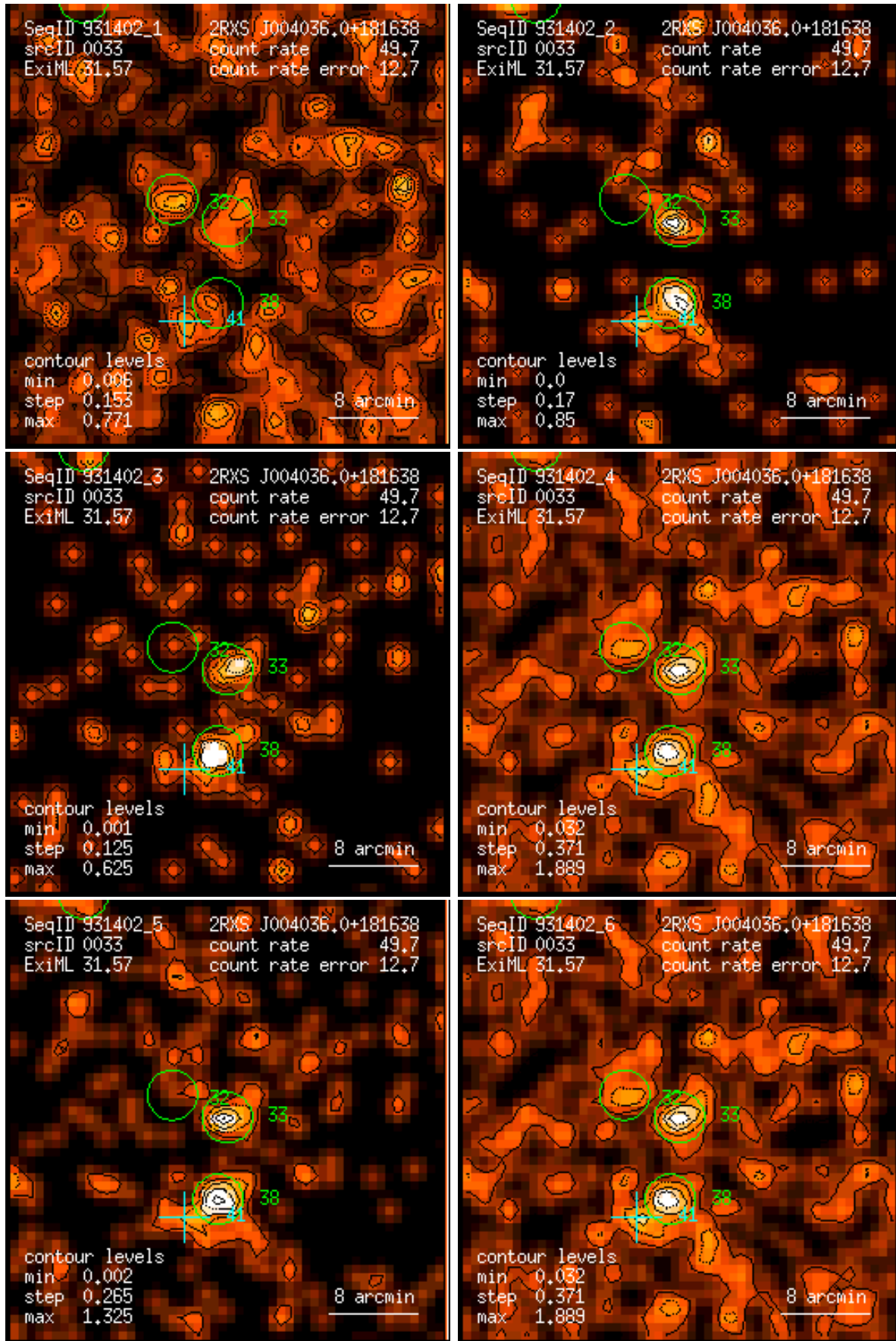
Figure 33: RASS 931402: detection 0033: band rate images, Gaussian filter: (1) PSPC channels 11 – 41, (2) 52 – 90, (3) 91 – 201, (4) 11 – 235, (5) 52 – 201, (6) 11 – 201. Broad band rates in counts/ks. Band rate contour levels in counts/ks/arcmin 2 .
