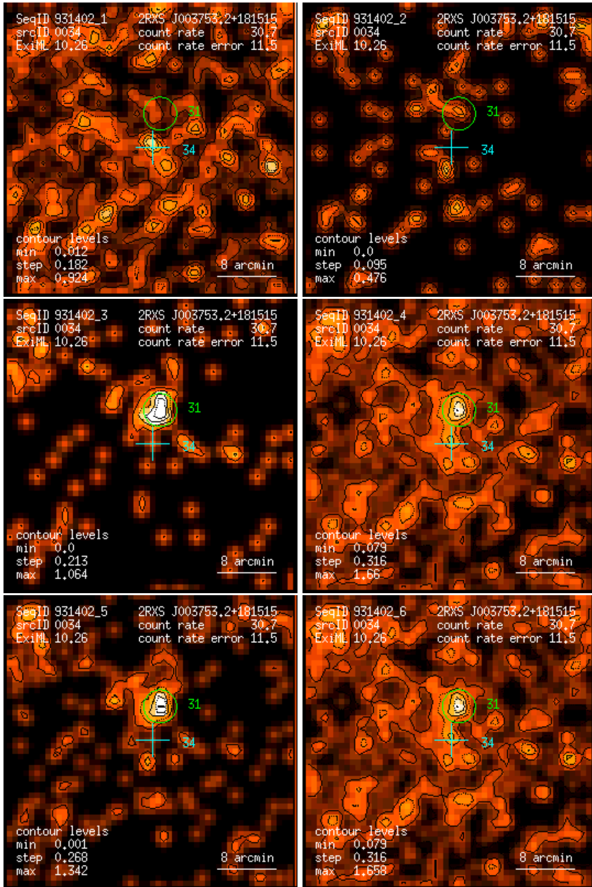
Figure 34: RASS 931402: detection 0034: band rate images, Gaussian filter: (1) PSPC channels 11 – 41, (2) 52 – 90, (3) 91 – 201, (4) 11 – 235, (5) 52 – 201, (6) 11 – 201. Broad band rates in counts/ks. Band rate contour levels in counts/ks/arcmin 2 .
