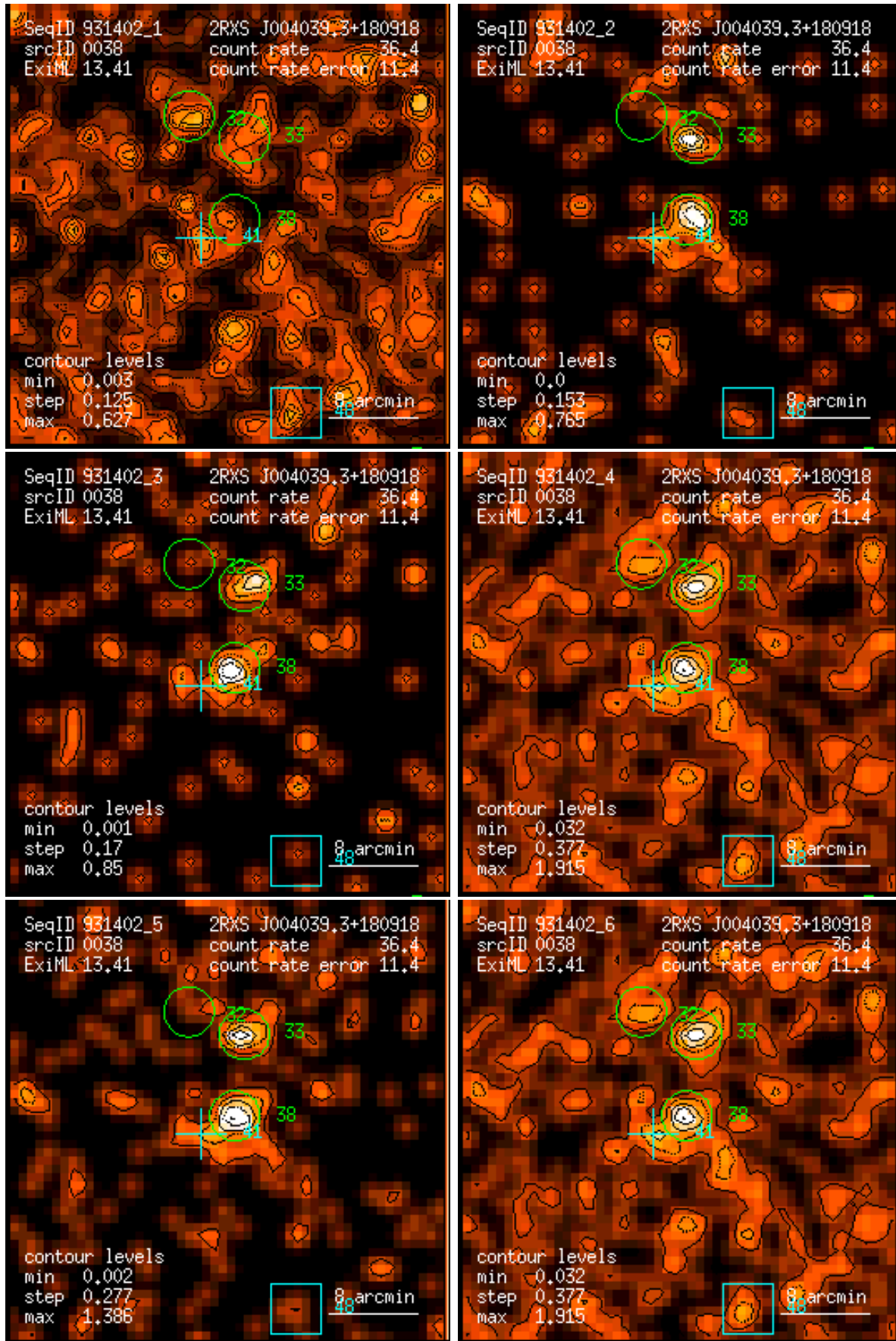
Figure 38: RASS 931402: detection 0038: band rate images, Gaussian filter: (1) PSPC channels 11 – 41, (2) 52 – 90, (3) 91 – 201, (4) 11 – 235, (5) 52 – 201, (6) 11 – 201. Broad band rates in counts/ks. Band rate contour levels in counts/ks/arcmin 2 .
