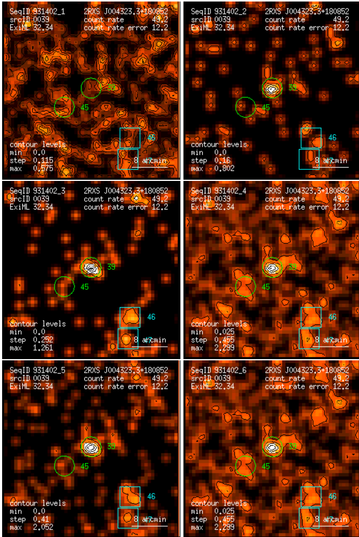
Figure 39: RASS 931402: detection 0039: band rate images, Gaussian filter: (1) PSPC channels 11 – 41, (2) 52 – 90, (3) 91 – 201, (4) 11 – 235, (5) 52 – 201, (6) 11 – 201. Broad band rates in counts/ks. Band rate contour levels in counts/ks/arcmin 2 .
