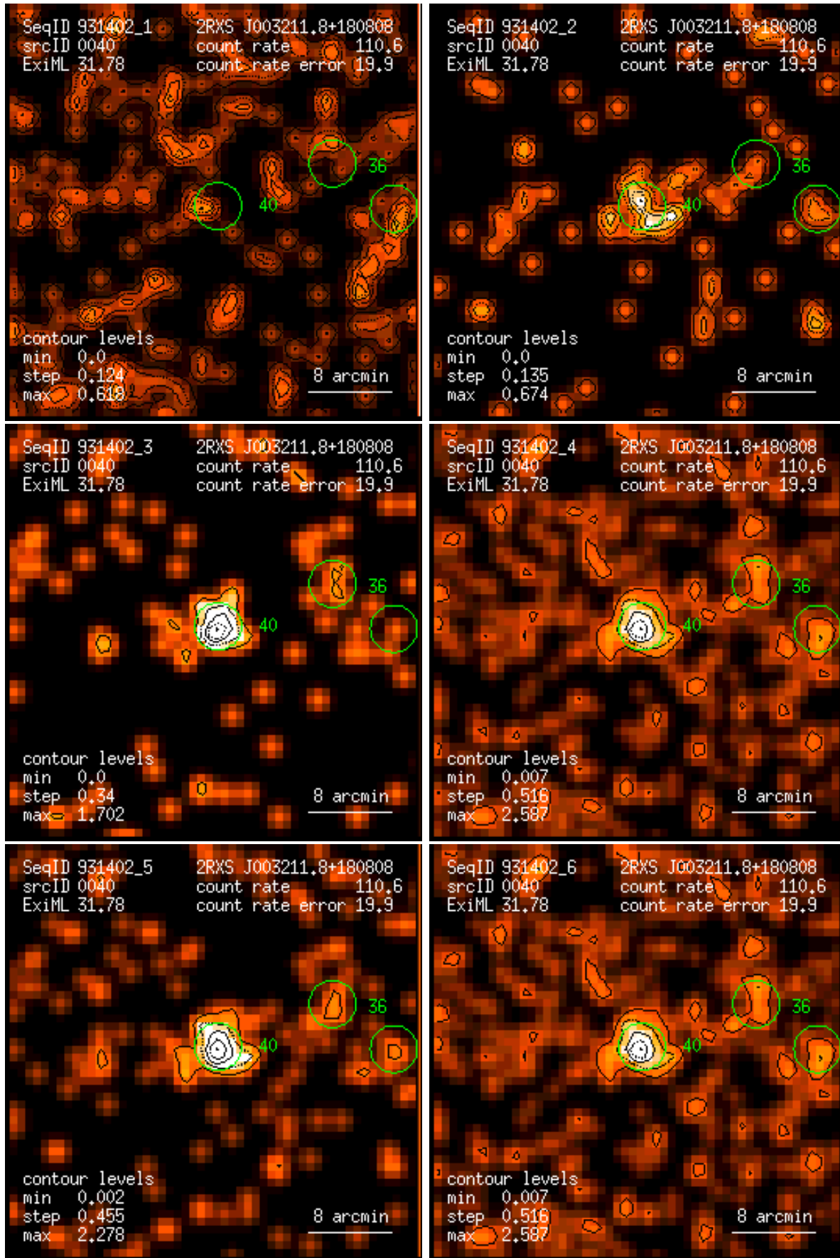
Figure 40: RASS 931402: detection 0040: band rate images, Gaussian filter: (1) PSPC channels 11 – 41, (2) 52 – 90, (3) 91 – 201, (4) 11 – 235, (5) 52 – 201, (6) 11 – 201. Broad band rates in counts/ks. Band rate contour levels in counts/ks/arcmin 2 .
