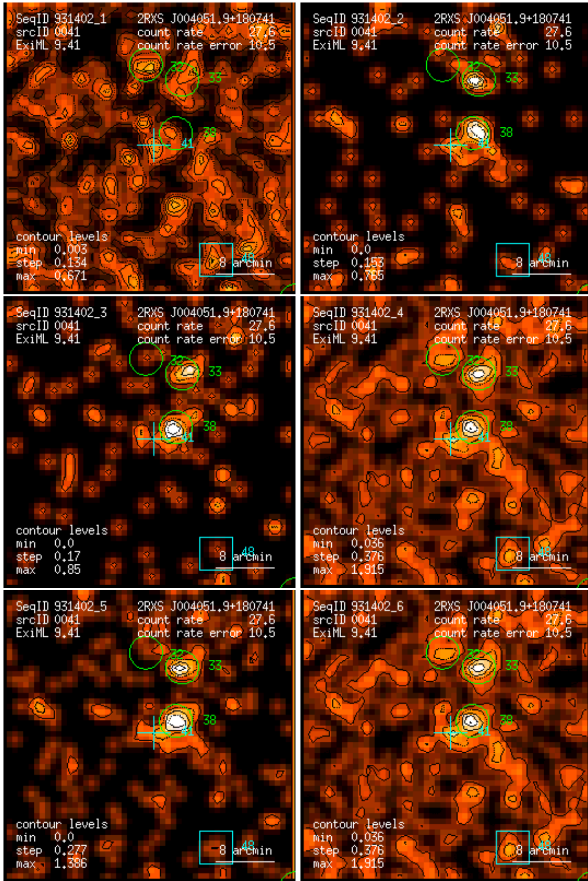
Figure 41: RASS 931402: detection 0041: band rate images, Gaussian filter: (1) PSPC channels 11 – 41, (2) 52 – 90, (3) 91 – 201, (4) 11 – 235, (5) 52 – 201, (6) 11 – 201. Broad band rates in counts/ks. Band rate contour levels in counts/ks/arcmin 2 .
