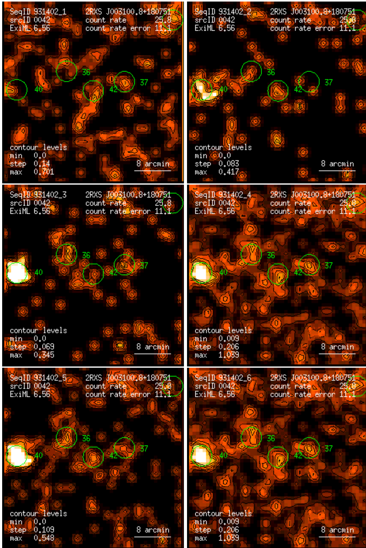
Figure 42: RASS 931402: detection 0042: band rate images, Gaussian filter: (1) PSPC channels 11 – 41, (2) 52 – 90, (3) 91 – 201, (4) 11 – 235, (5) 52 – 201, (6) 11 – 201. Broad band rates in counts/ks. Band rate contour levels in counts/ks/arcmin 2 .
