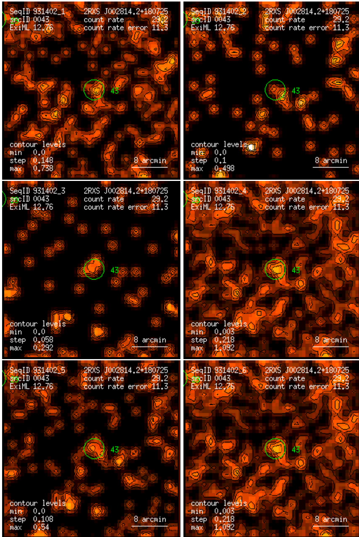
Figure 43: RASS 931402: detection 0043: band rate images, Gaussian filter: (1) PSPC channels 11 – 41, (2) 52 – 90, (3) 91 – 201, (4) 11 – 235, (5) 52 – 201, (6) 11 – 201. Broad band rates in counts/ks. Band rate contour levels in counts/ks/arcmin 2 .
