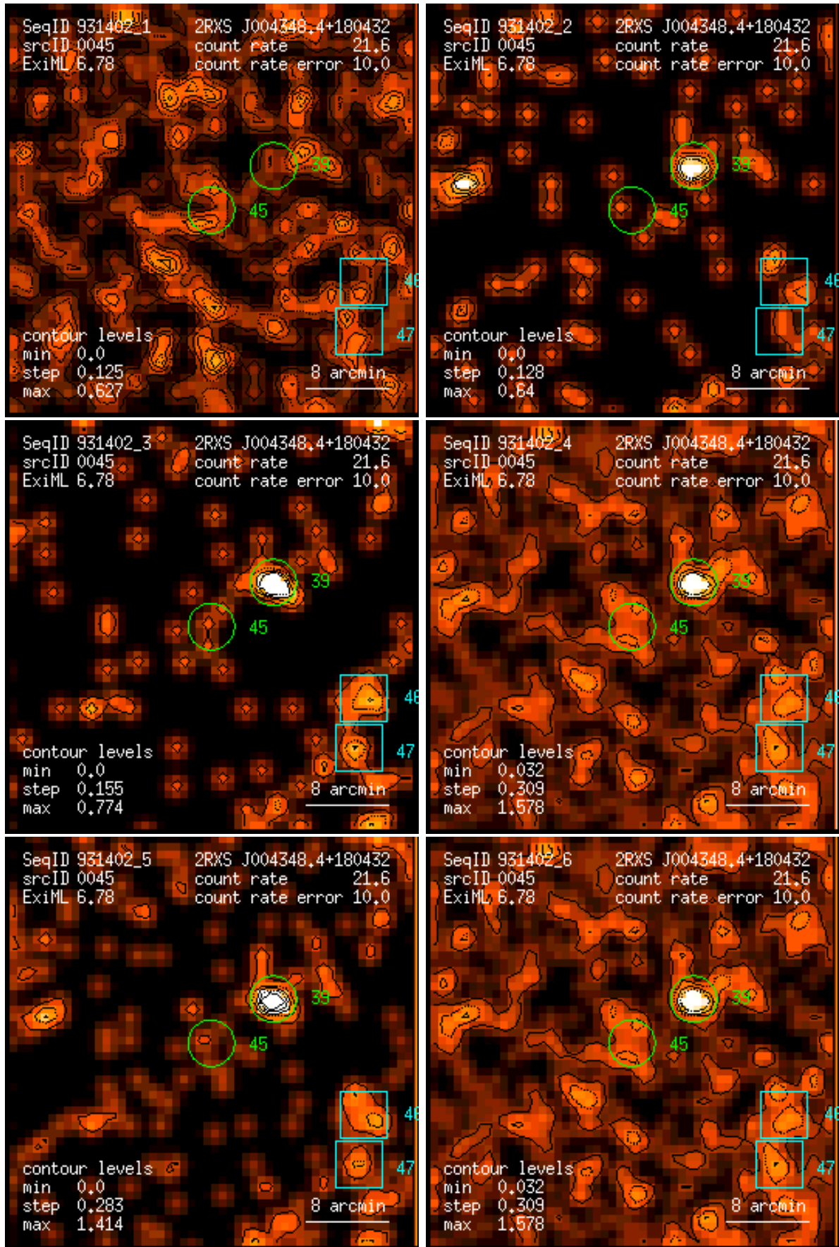
Figure 45: RASS 931402: detection 0045: band rate images, Gaussian filter: (1) PSPC channels 11 – 41, (2) 52 – 90, (3) 91 – 201, (4) 11 – 235, (5) 52 – 201, (6) 11 – 201. Broad band rates in counts/ks. Band rate contour levels in counts/ks/arcmin 2 .
