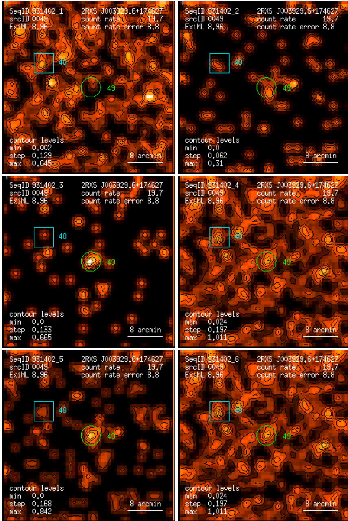
Figure 49: RASS 931402: detection 0049: band rate images, Gaussian filter: (1) PSPC channels 11 – 41, (2) 52 – 90, (3) 91 – 201, (4) 11 – 235, (5) 52 – 201, (6) 11 – 201. Broad band rates in counts/ks. Band rate contour levels in counts/ks/arcmin 2 .
