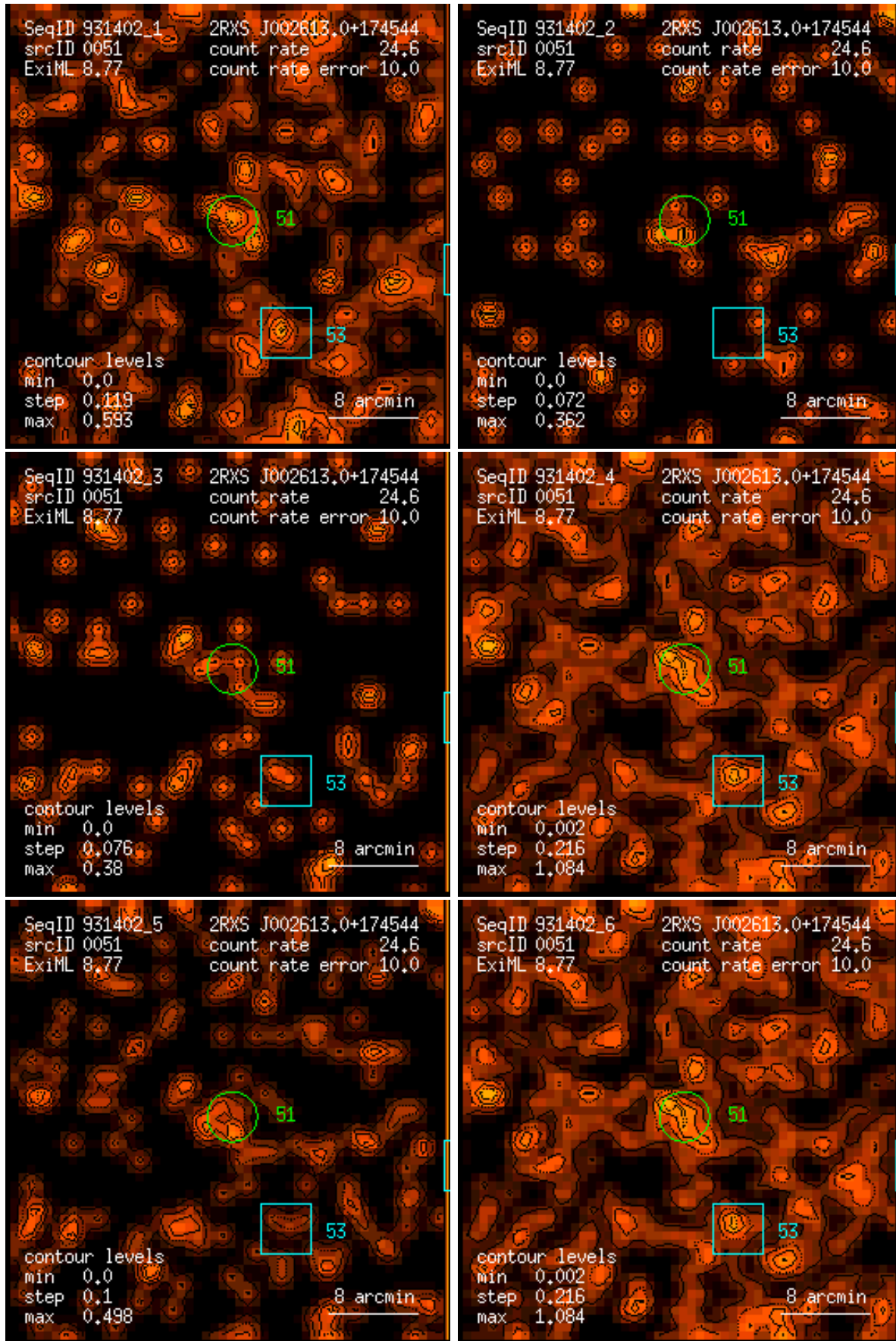
Figure 51: RASS 931402: detection 0051: band rate images, Gaussian filter: (1) PSPC channels 11 – 41, (2) 52 – 90, (3) 91 – 201, (4) 11 – 235, (5) 52 – 201, (6) 11 – 201. Broad band rates in counts/ks. Band rate contour levels in counts/ks/arcmin 2 .
