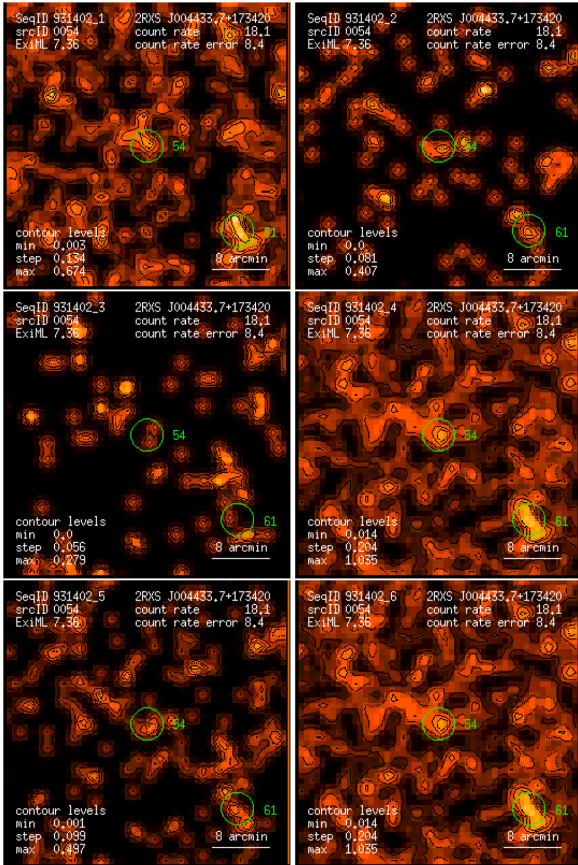
Figure 54: RASS 931402: detection 0054: band rate images, Gaussian filter: (1) PSPC channels 11 – 41, (2) 52 – 90, (3) 91 – 201, (4) 11 – 235, (5) 52 – 201, (6) 11 – 201. Broad band rates in counts/ks. Band rate contour levels in counts/ks/arcmin 2 .
