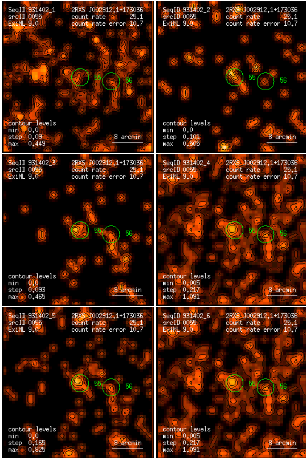
Figure 55: RASS 931402: detection 0055: band rate images, Gaussian filter: (1) PSPC channels 11 – 41, (2) 52 – 90, (3) 91 – 201, (4) 11 – 235, (5) 52 – 201, (6) 11 – 201. Broad band rates in counts/ks. Band rate contour levels in counts/ks/arcmin 2 .
