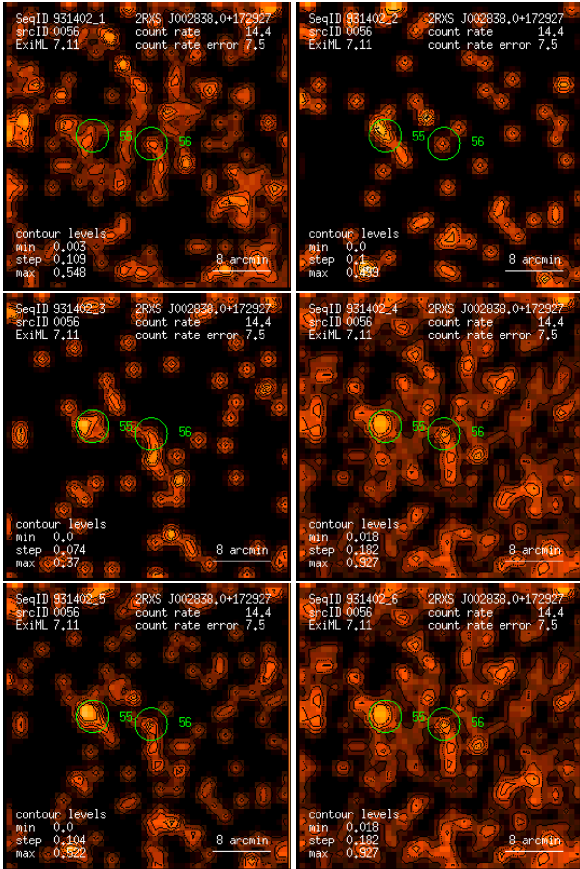
Figure 56: RASS 931402: detection 0056: band rate images, Gaussian filter: (1) PSPC channels 11 – 41, (2) 52 – 90, (3) 91 – 201, (4) 11 – 235, (5) 52 – 201, (6) 11 – 201. Broad band rates in counts/ks. Band rate contour levels in counts/ks/arcmin 2 .
