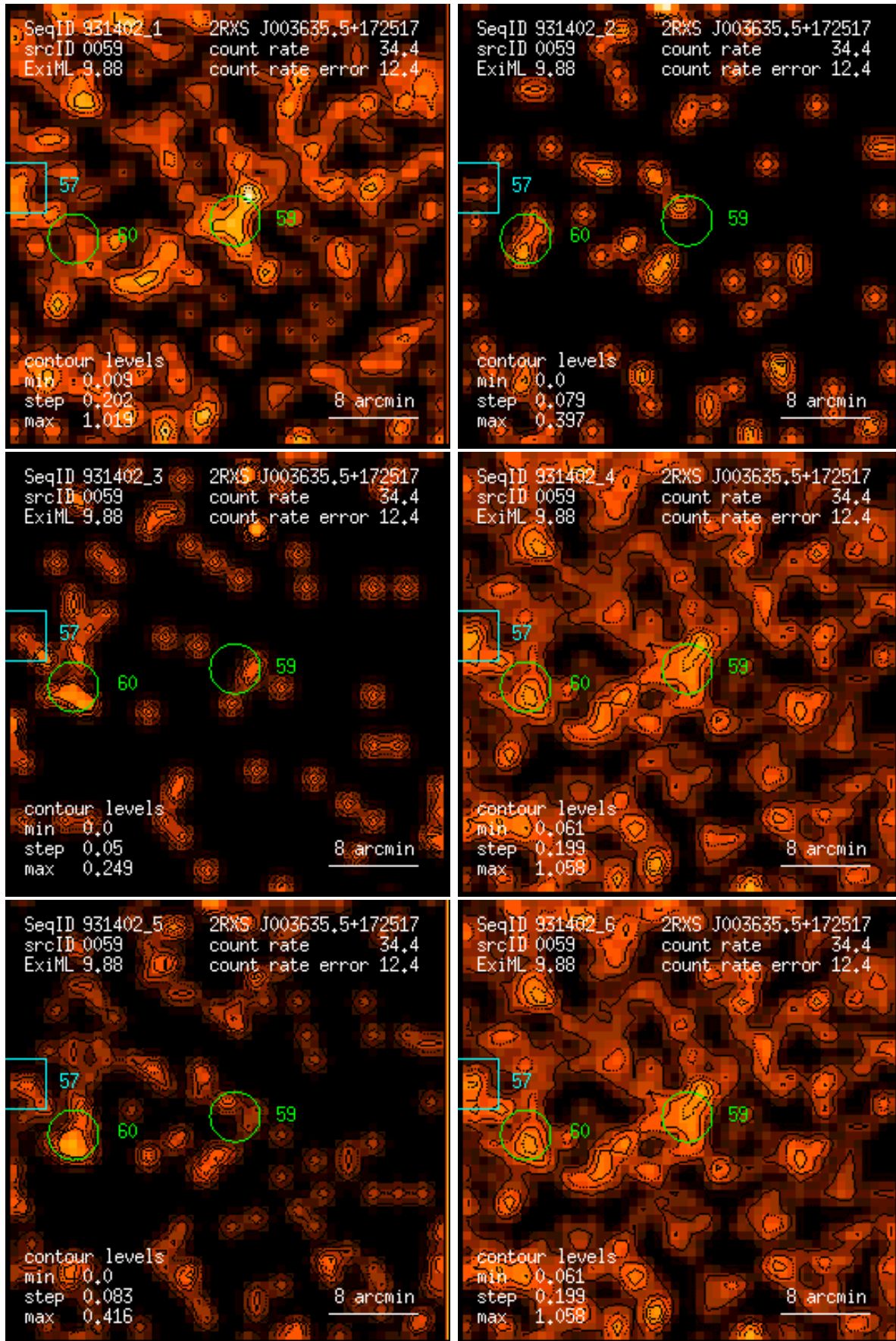
Figure 59: RASS 931402: detection 0059: band rate images, Gaussian filter: (1) PSPC channels 11 – 41, (2) 52 – 90, (3) 91 – 201, (4) 11 – 235, (5) 52 – 201, (6) 11 – 201. Broad band rates in counts/ks. Band rate contour levels in counts/ks/arcmin 2 .
