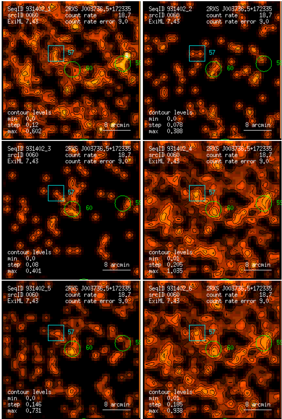
Figure 60: RASS 931402: detection 0060: band rate images, Gaussian filter: (1) PSPC channels 11 – 41, (2) 52 – 90, (3) 91 – 201, (4) 11 – 235, (5) 52 – 201, (6) 11 – 201. Broad band rates in counts/ks. Band rate contour levels in counts/ks/arcmin 2 .
