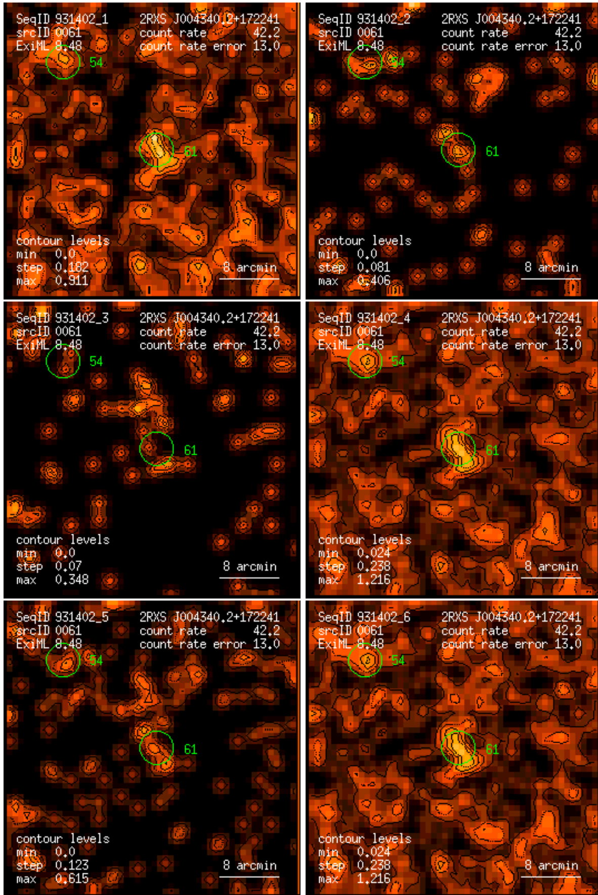
Figure 61: RASS 931402: detection 0061: band rate images, Gaussian filter: (1) PSPC channels 11 – 41, (2) 52 – 90, (3) 91 – 201, (4) 11 – 235, (5) 52 – 201, (6) 11 – 201. Broad band rates in counts/ks. Band rate contour levels in counts/ks/arcmin 2 .
