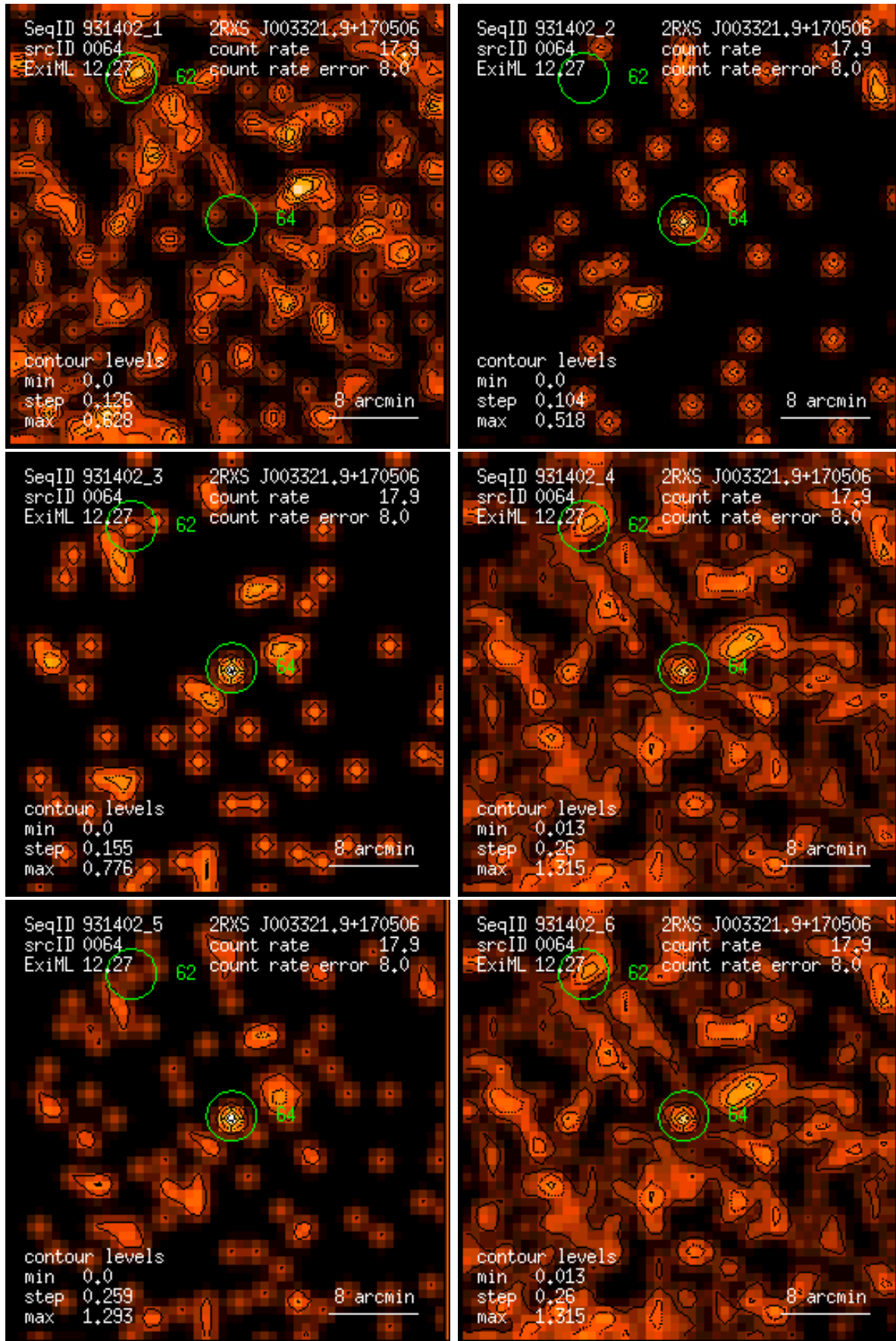
Figure 64: RASS 931402: detection 0064: band rate images, Gaussian filter: (1) PSPC channels 11 – 41, (2) 52 – 90, (3) 91 – 201, (4) 11 – 235, (5) 52 – 201, (6) 11 – 201. Broad band rates in counts/ks. Band rate contour levels in counts/ks/arcmin 2 .
