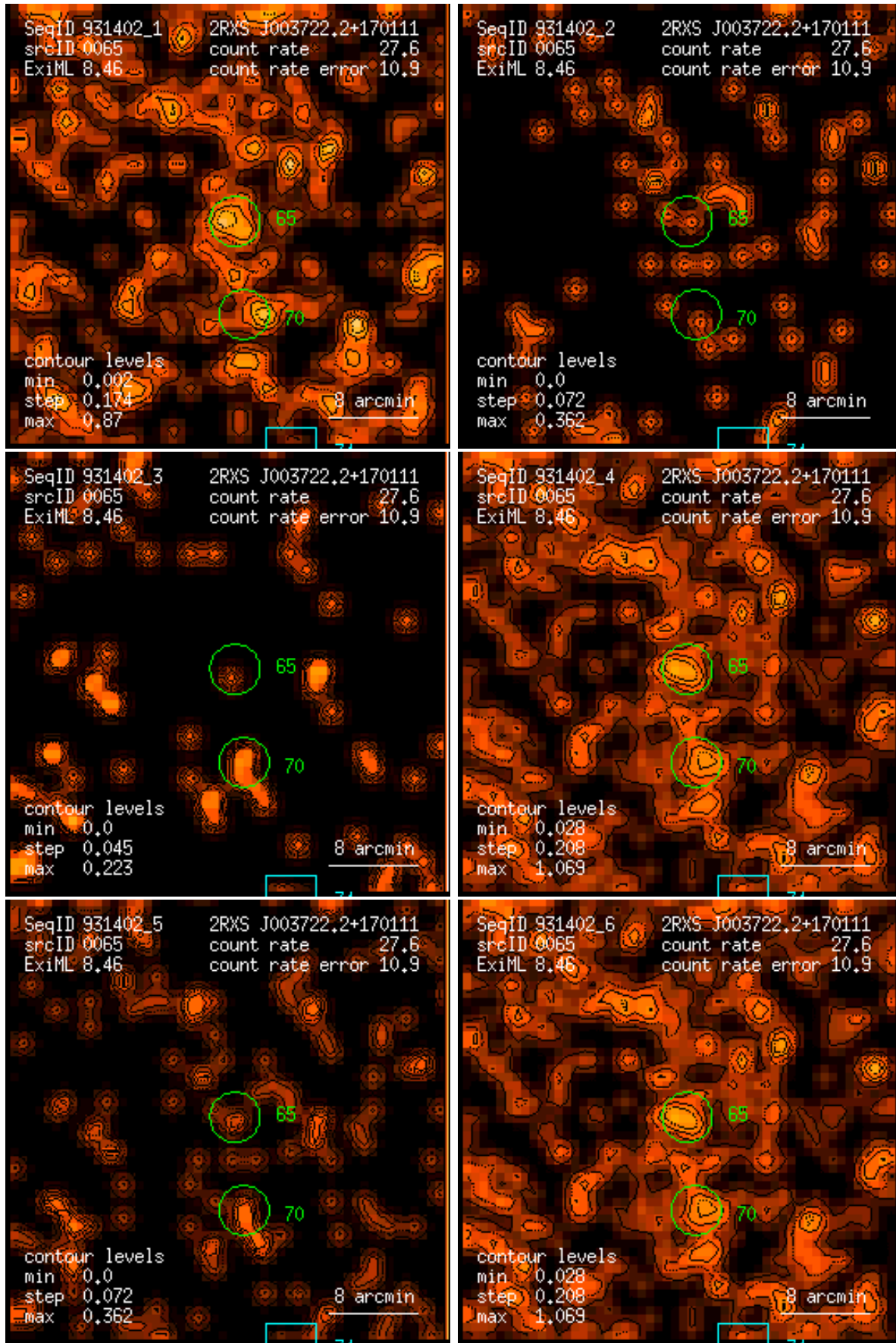
Figure 65: RASS 931402: detection 0065: band rate images, Gaussian filter: (1) PSPC channels 11 – 41, (2) 52 – 90, (3) 91 – 201, (4) 11 – 235, (5) 52 – 201, (6) 11 – 201. Broad band rates in counts/ks. Band rate contour levels in counts/ks/arcmin 2 .
