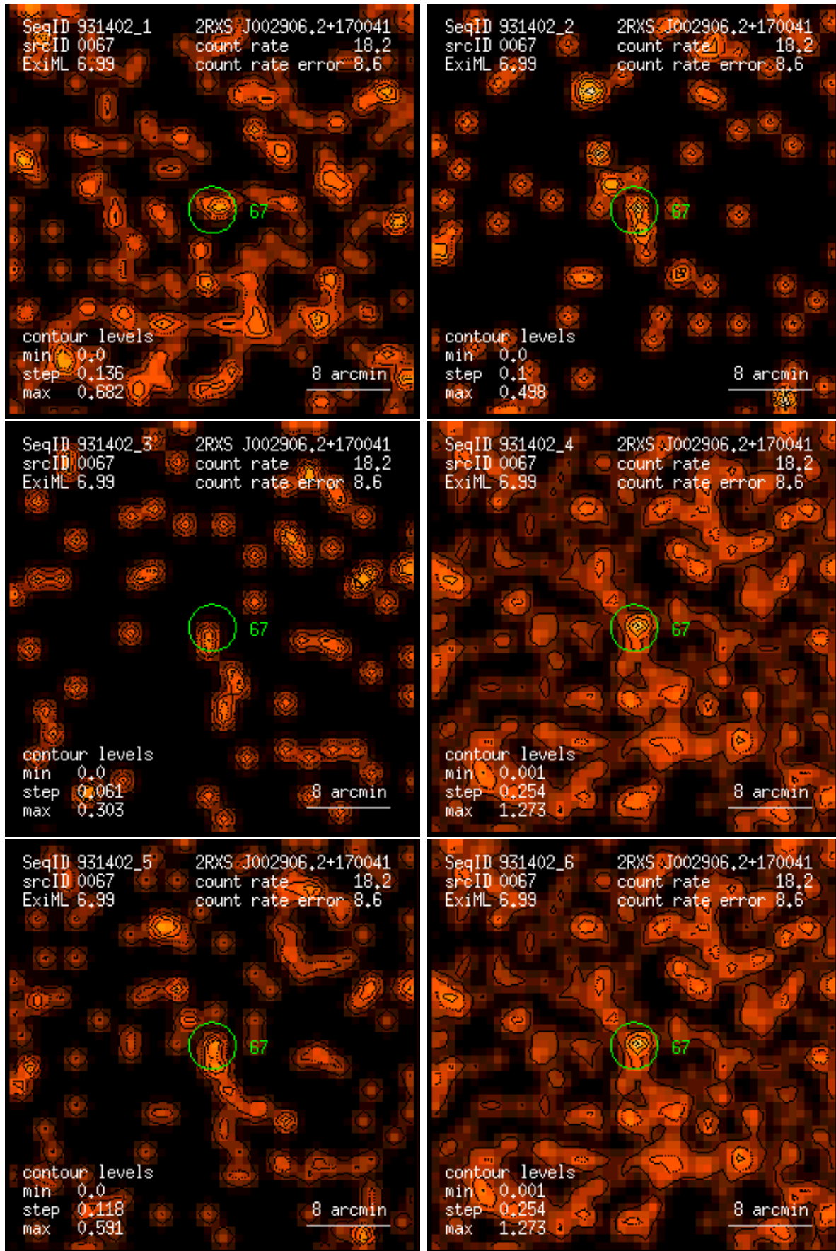
Figure 67: RASS 931402: detection 0067: band rate images, Gaussian filter: (1) PSPC channels 11 – 41, (2) 52 – 90, (3) 91 – 201, (4) 11 – 235, (5) 52 – 201, (6) 11 – 201. Broad band rates in counts/ks. Band rate contour levels in counts/ks/arcmin 2 .
