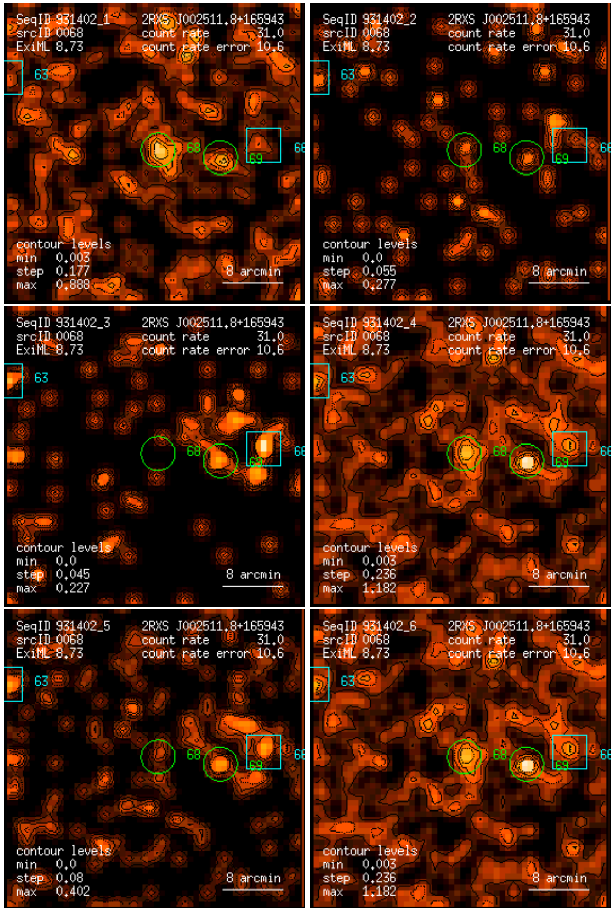
Figure 68: RASS 931402: detection 0068: band rate images, Gaussian filter: (1) PSPC channels 11 – 41, (2) 52 – 90, (3) 91 – 201, (4) 11 – 235, (5) 52 – 201, (6) 11 – 201. Broad band rates in counts/ks. Band rate contour levels in counts/ks/arcmin 2 .
