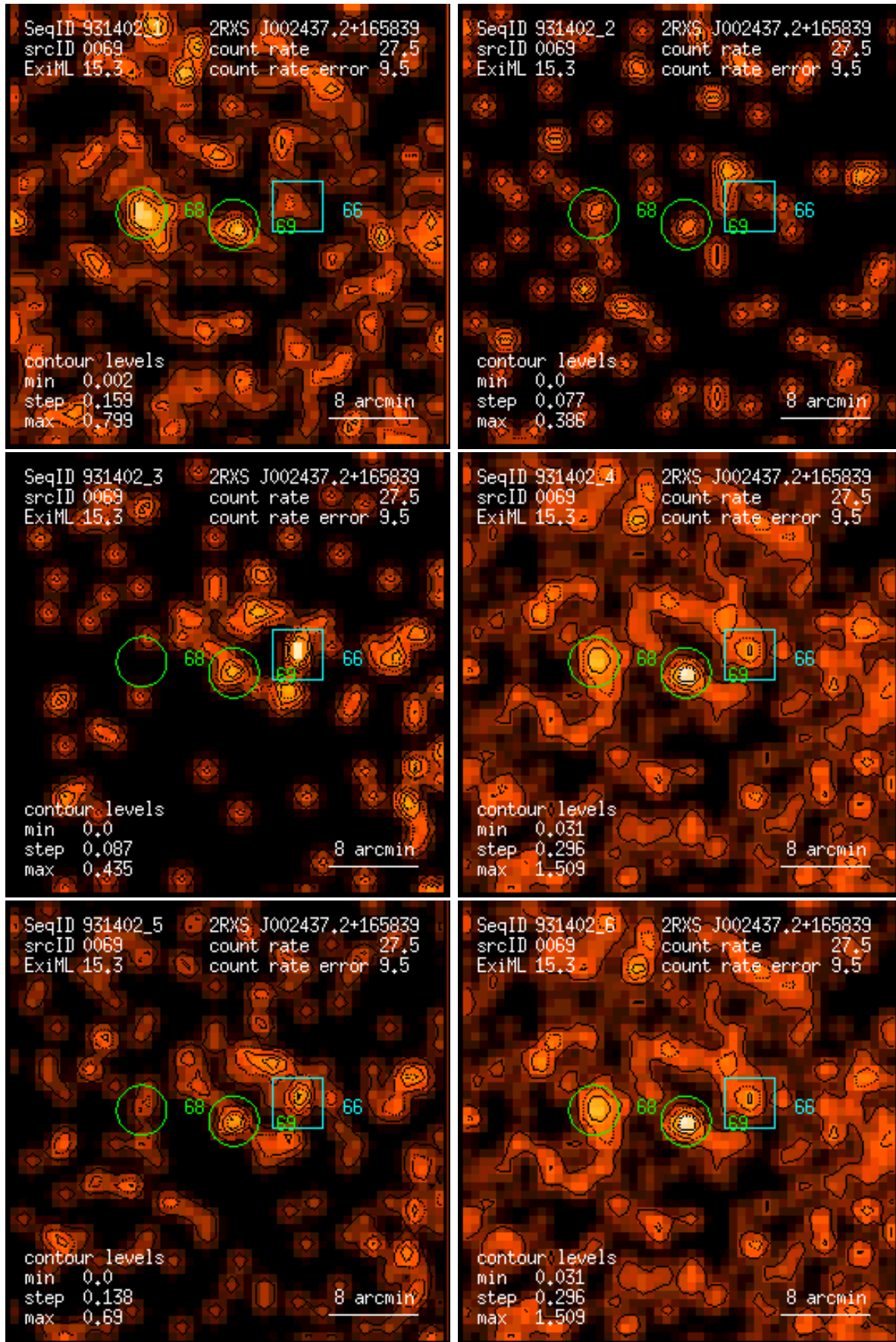
Figure 69: RASS 931402: detection 0069: band rate images, Gaussian filter: (1) PSPC channels 11 – 41, (2) 52 – 90, (3) 91 – 201, (4) 11 – 235, (5) 52 – 201, (6) 11 – 201. Broad band rates in counts/ks. Band rate contour levels in counts/ks/arcmin 2 .
