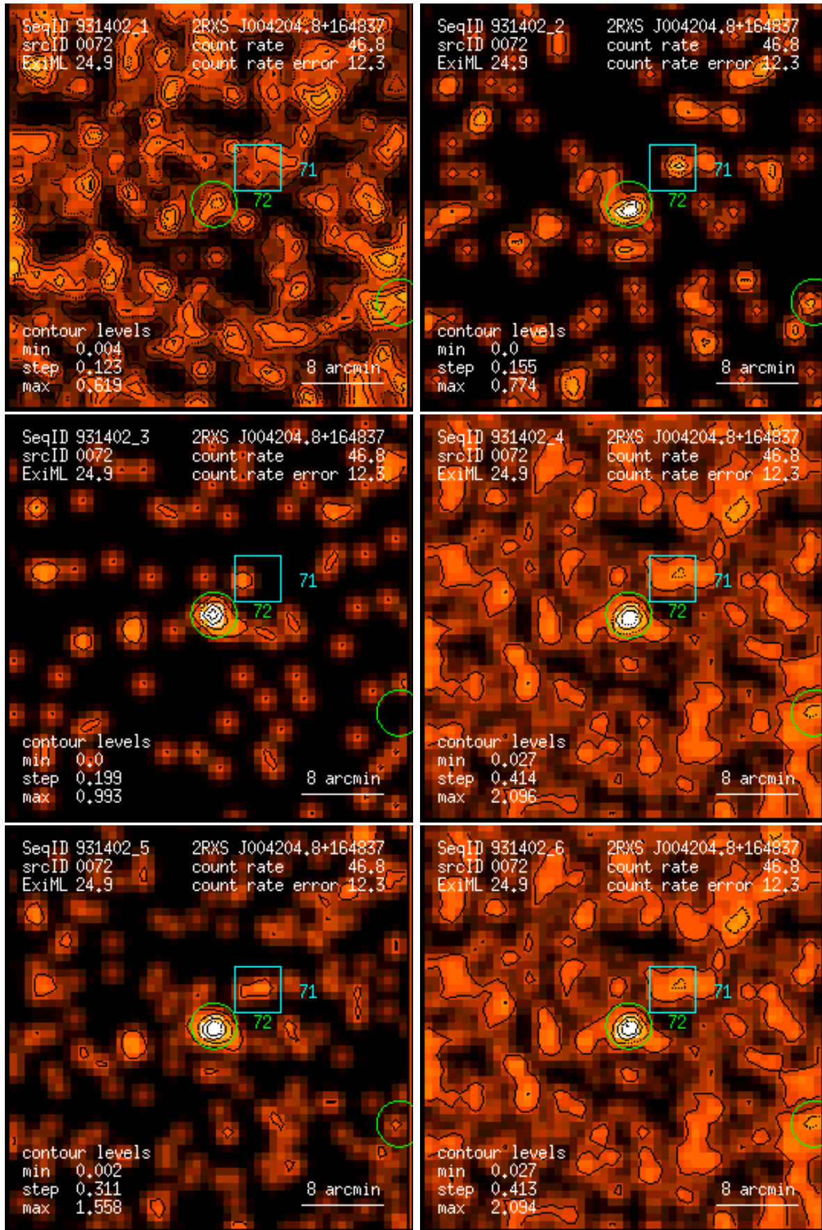
Figure 72: RASS 931402: detection 0072: band rate images, Gaussian filter: (1) PSPC channels 11 – 41, (2) 52 – 90, (3) 91 – 201, (4) 11 – 235, (5) 52 – 201, (6) 11 – 201. Broad band rates in counts/ks. Band rate contour levels in counts/ks/arcmin 2 .
