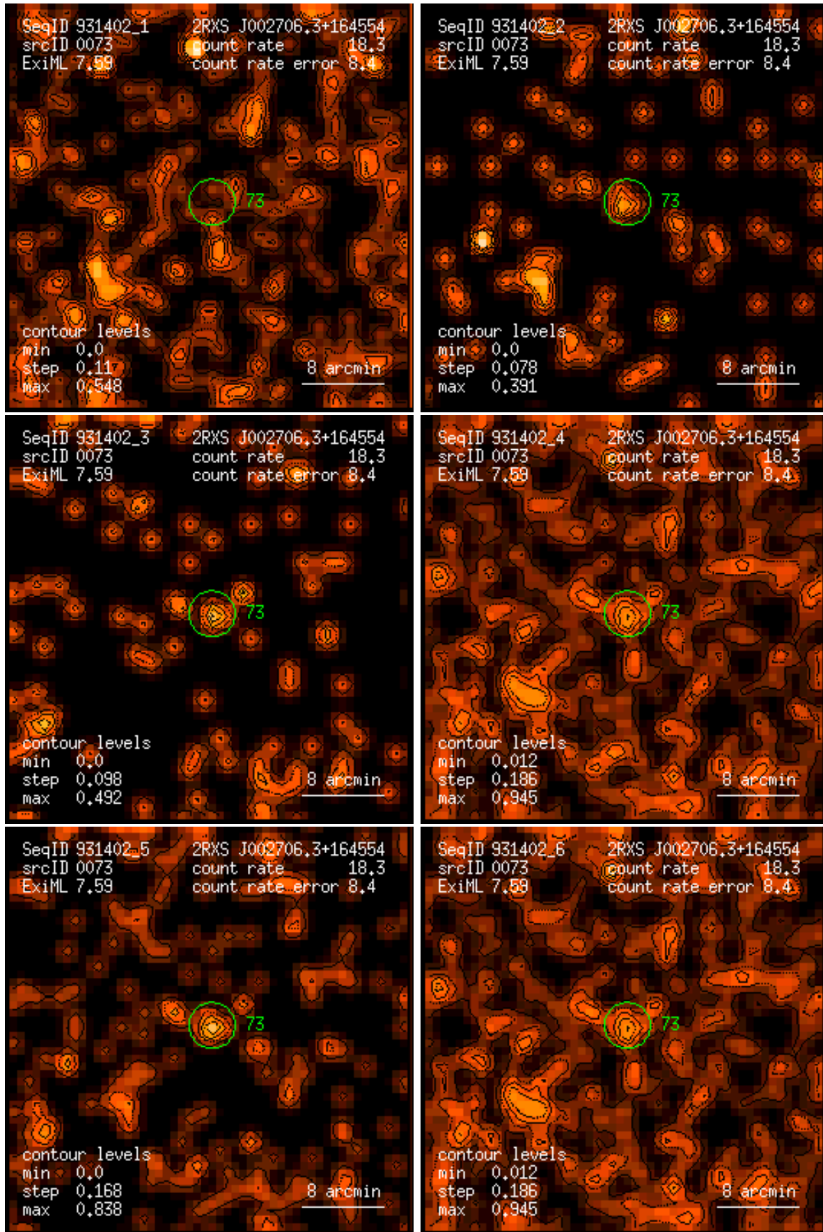
Figure 73: RASS 931402: detection 0073: band rate images, Gaussian filter: (1) PSPC channels 11 – 41, (2) 52 – 90, (3) 91 – 201, (4) 11 – 235, (5) 52 – 201, (6) 11 – 201. Broad band rates in counts/ks. Band rate contour levels in counts/ks/arcmin 2 .
