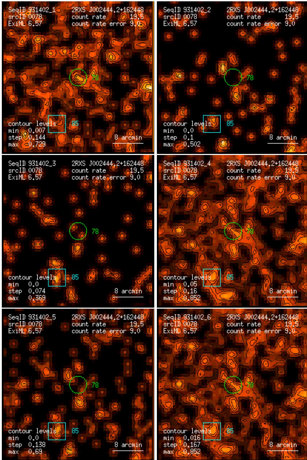
Figure 78: RASS 931402: detection 0078: band rate images, Gaussian filter: (1) PSPC channels 11 – 41, (2) 52 – 90, (3) 91 – 201, (4) 11 – 235, (5) 52 – 201, (6) 11 – 201. Broad band rates in counts/ks. Band rate contour levels in counts/ks/arcmin 2 .
