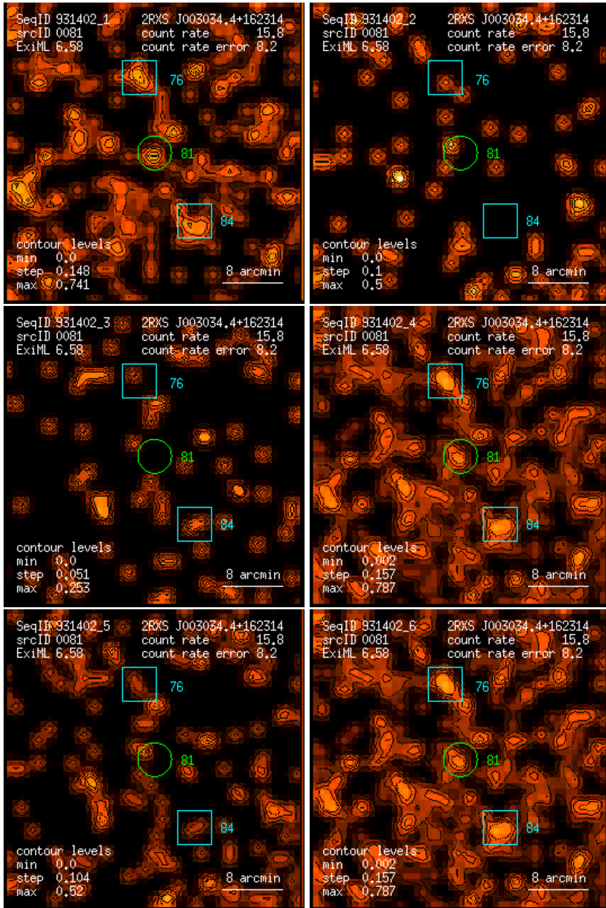
Figure 81: RASS 931402: detection 0081: band rate images, Gaussian filter: (1) PSPC channels 11 – 41, (2) 52 – 90, (3) 91 – 201, (4) 11 – 235, (5) 52 – 201, (6) 11 – 201. Broad band rates in counts/ks. Band rate contour levels in counts/ks/arcmin 2 .
