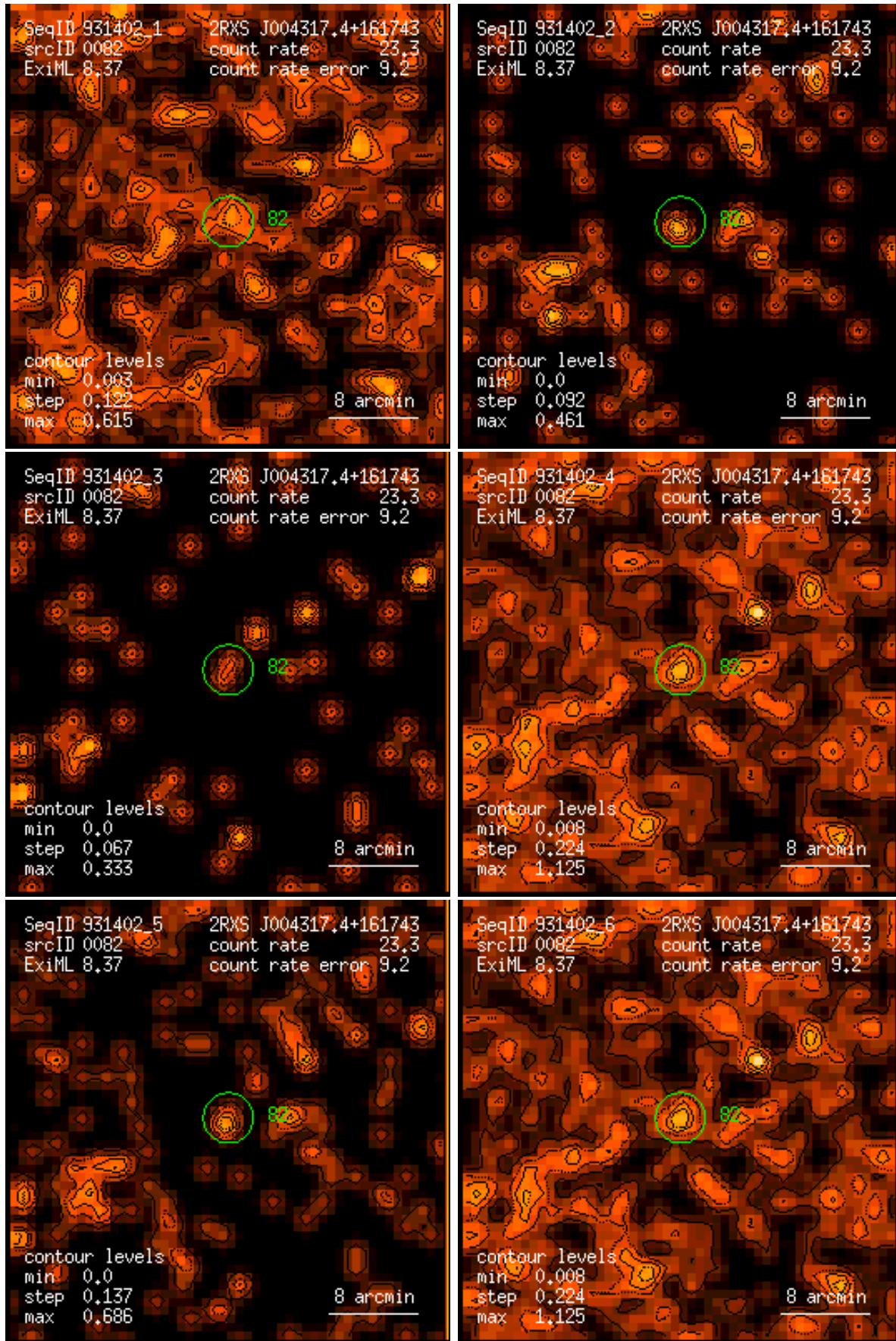
Figure 82: RASS 931402: detection 0082: band rate images, Gaussian filter: (1) PSPC channels 11 – 41, (2) 52 – 90, (3) 91 – 201, (4) 11 – 235, (5) 52 – 201, (6) 11 – 201. Broad band rates in counts/ks. Band rate contour levels in counts/ks/arcmin 2 .
