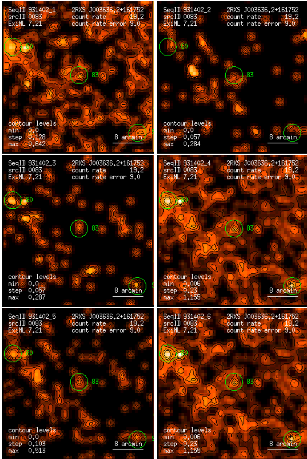
Figure 83: RASS 931402: detection 0083: band rate images, Gaussian filter: (1) PSPC channels 11 – 41, (2) 52 – 90, (3) 91 – 201, (4) 11 – 235, (5) 52 – 201, (6) 11 – 201. Broad band rates in counts/ks. Band rate contour levels in counts/ks/arcmin 2 .
