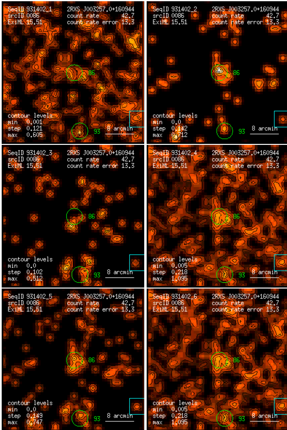
Figure 86: RASS 931402: detection 0086: band rate images, Gaussian filter: (1) PSPC channels 11 – 41, (2) 52 – 90, (3) 91 – 201, (4) 11 – 235, (5) 52 – 201, (6) 11 – 201. Broad band rates in counts/ks. Band rate contour levels in counts/ks/arcmin 2 .
