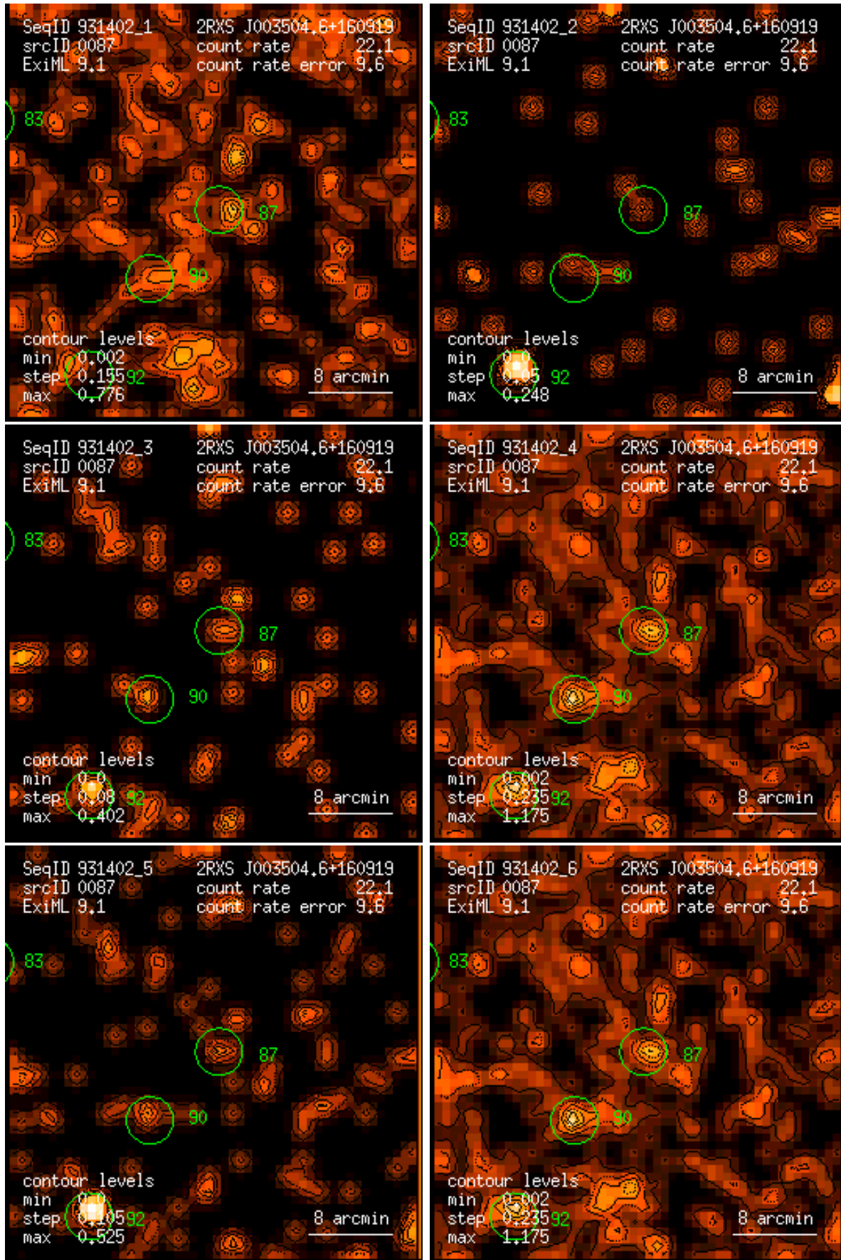
Figure 87: RASS 931402: detection 0087: band rate images, Gaussian filter: (1) PSPC channels 11 – 41, (2) 52 – 90, (3) 91 – 201, (4) 11 – 235, (5) 52 – 201, (6) 11 – 201. Broad band rates in counts/ks. Band rate contour levels in counts/ks/arcmin 2 .
