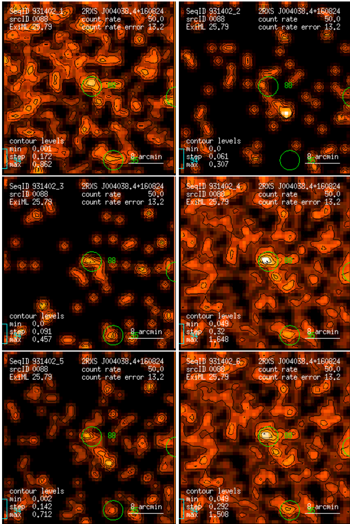
Figure 88: RASS 931402: detection 0088: band rate images, Gaussian filter: (1) PSPC channels 11 – 41, (2) 52 – 90, (3) 91 – 201, (4) 11 – 235, (5) 52 – 201, (6) 11 – 201. Broad band rates in counts/ks. Band rate contour levels in counts/ks/arcmin 2 .
