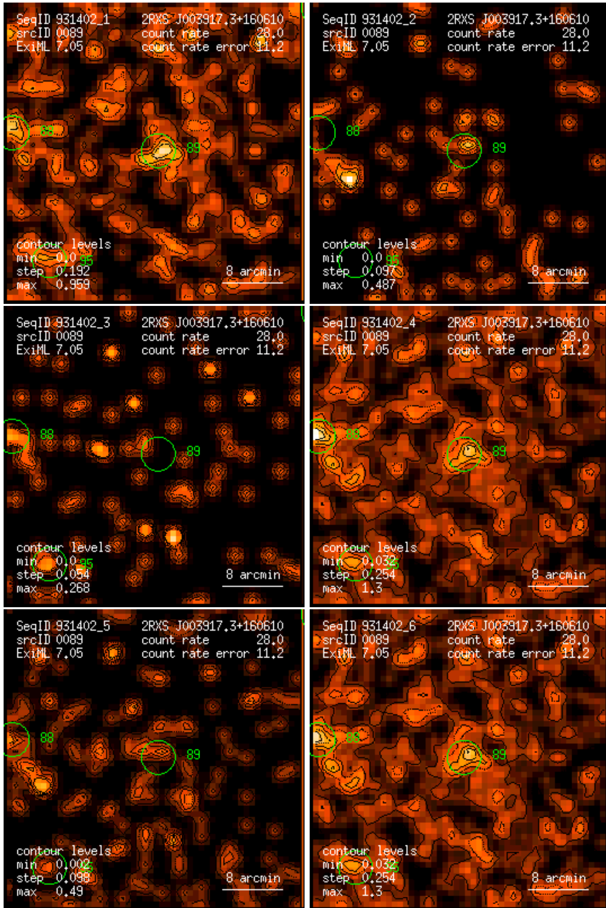
Figure 89: RASS 931402: detection 0089: band rate images, Gaussian filter: (1) PSPC channels 11 – 41, (2) 52 – 90, (3) 91 – 201, (4) 11 – 235, (5) 52 – 201, (6) 11 – 201. Broad band rates in counts/ks. Band rate contour levels in counts/ks/arcmin 2 .
