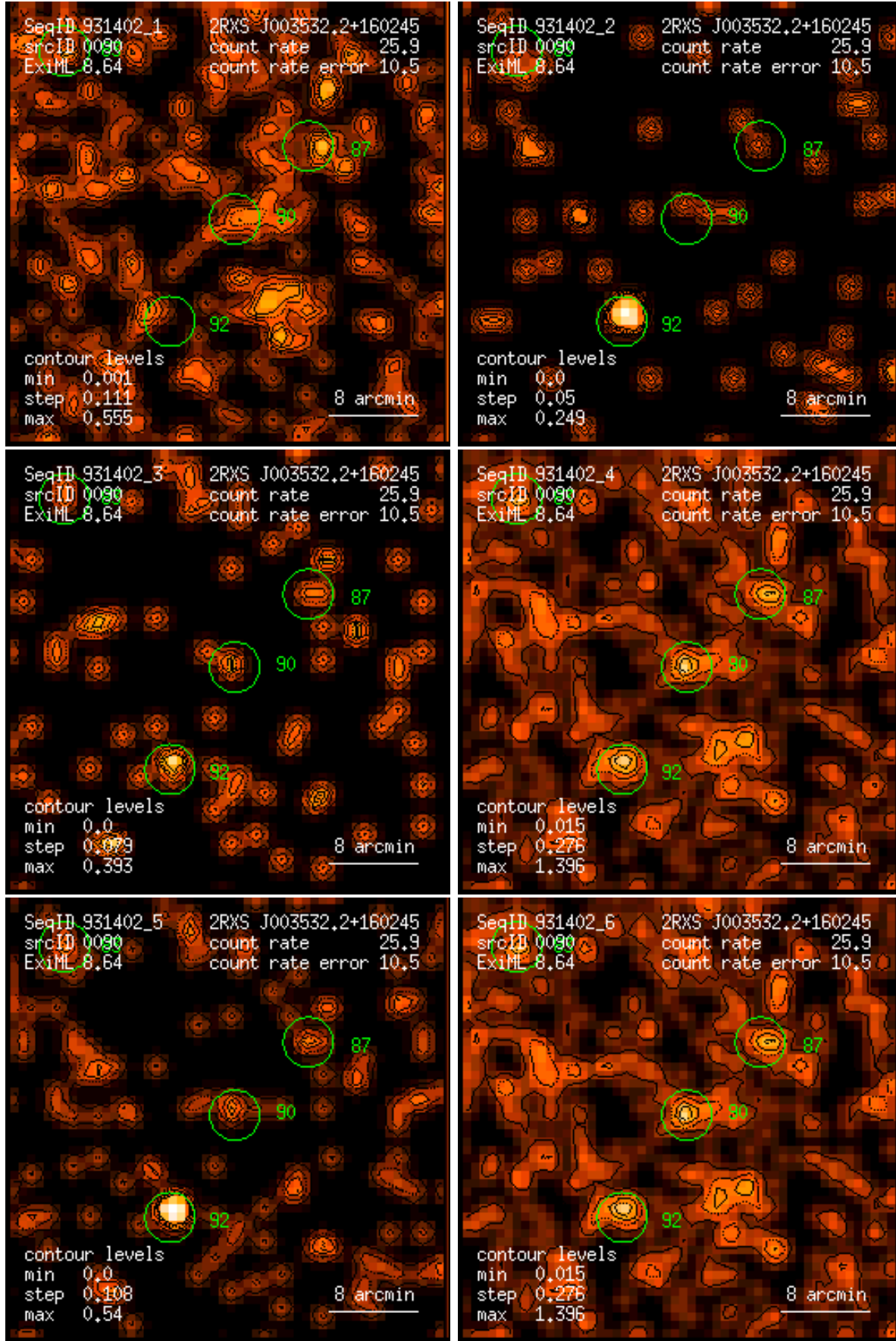
Figure 90: RASS 931402: detection 0090: band rate images, Gaussian filter: (1) PSPC channels 11 – 41, (2) 52 – 90, (3) 91 – 201, (4) 11 – 235, (5) 52 – 201, (6) 11 – 201. Broad band rates in counts/ks. Band rate contour levels in counts/ks/arcmin 2 .
