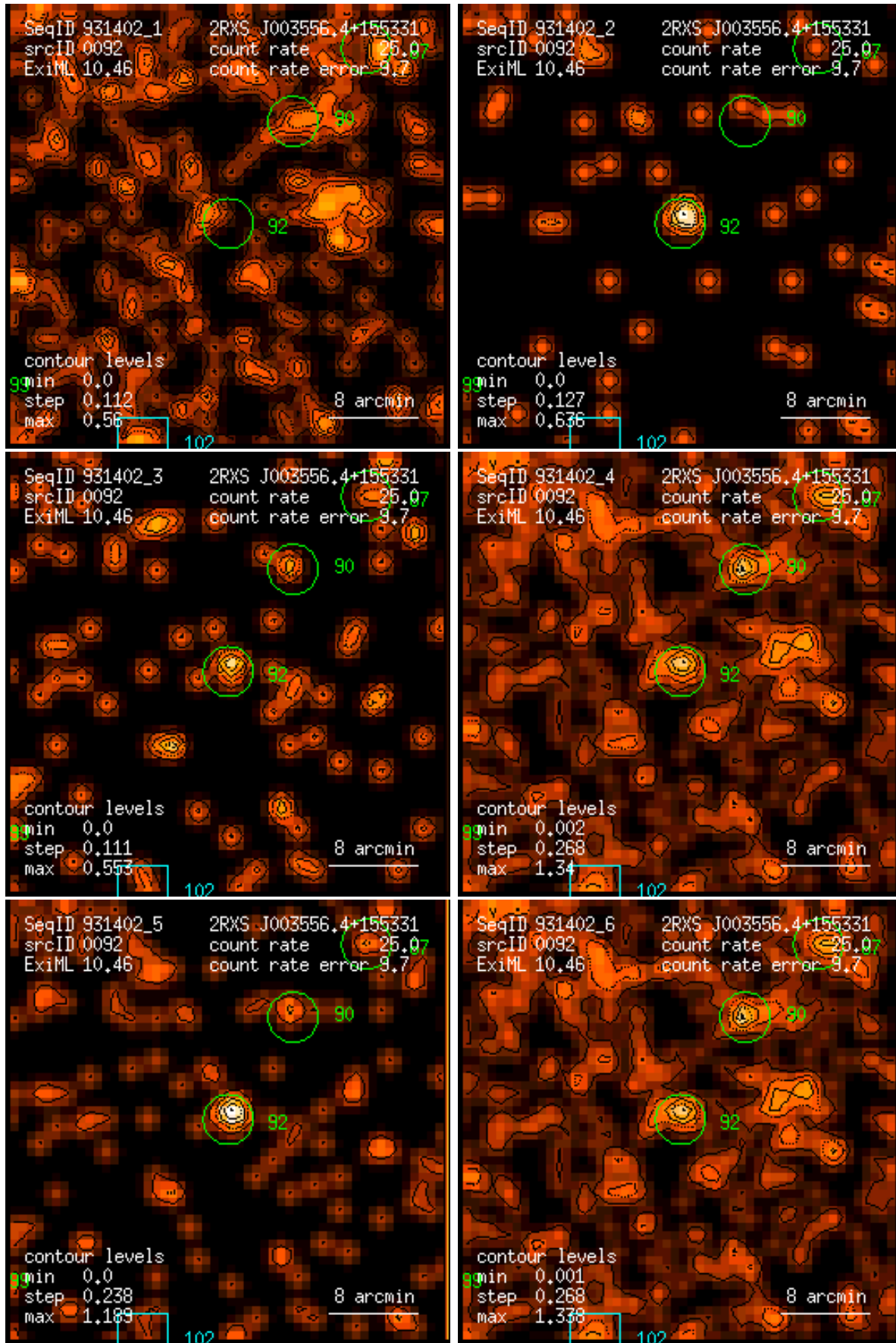
Figure 92: RASS 931402: detection 0092: band rate images, Gaussian filter: (1) PSPC channels 11 – 41, (2) 52 – 90, (3) 91 – 201, (4) 11 – 235, (5) 52 – 201, (6) 11 – 201. Broad band rates in counts/ks. Band rate contour levels in counts/ks/arcmin 2 .
