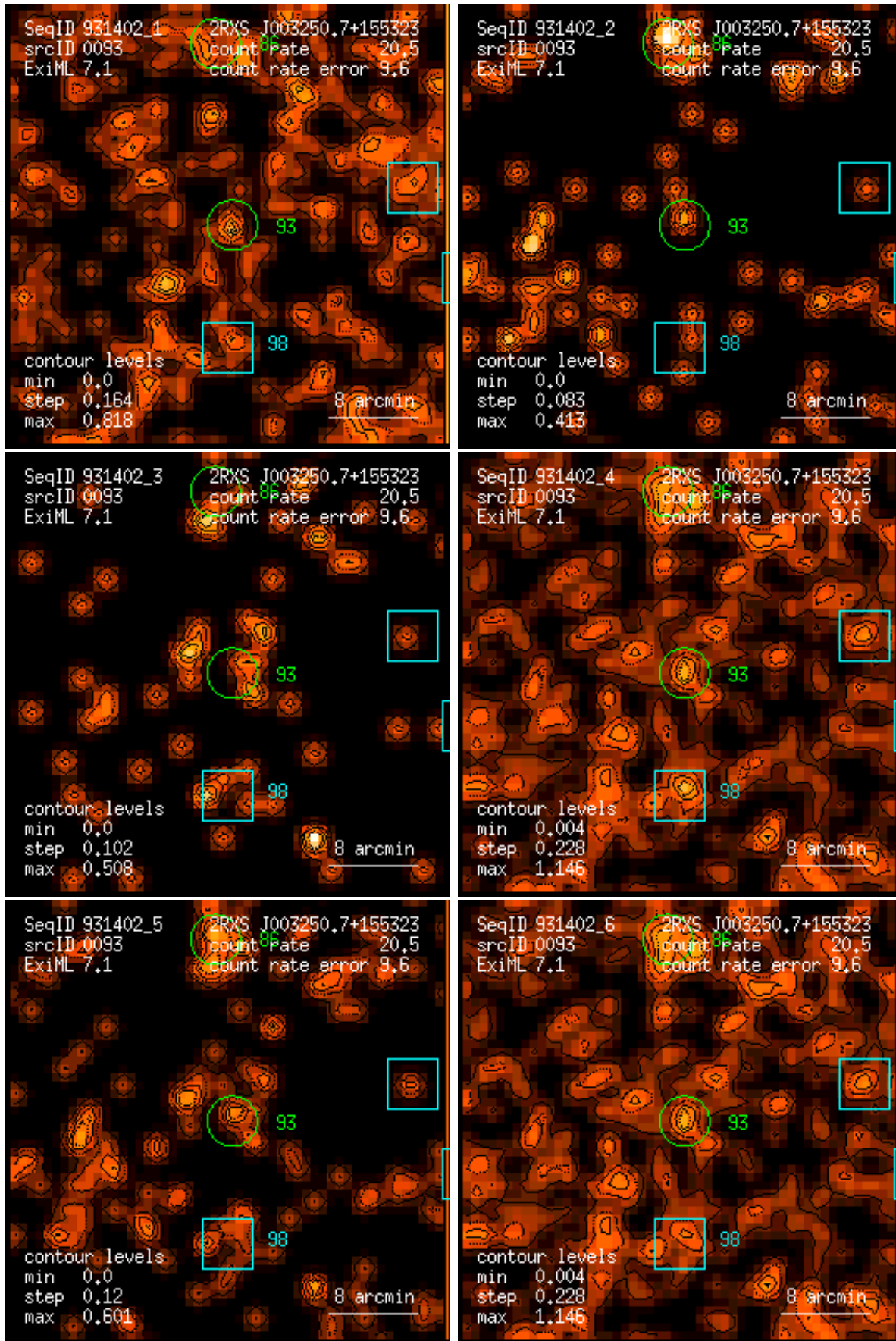
Figure 93: RASS 931402: detection 0093: band rate images, Gaussian filter: (1) PSPC channels 11 – 41, (2) 52 – 90, (3) 91 – 201, (4) 11 – 235, (5) 52 – 201, (6) 11 – 201. Broad band rates in counts/ks. Band rate contour levels in counts/ks/arcmin 2 .
